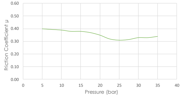
Pressure Sensitivity
