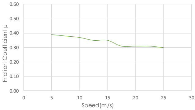
Speed Sensitivity
