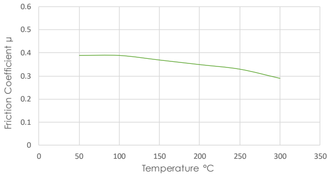
Temperature Sensitivity
