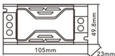
RG-24V-60W
