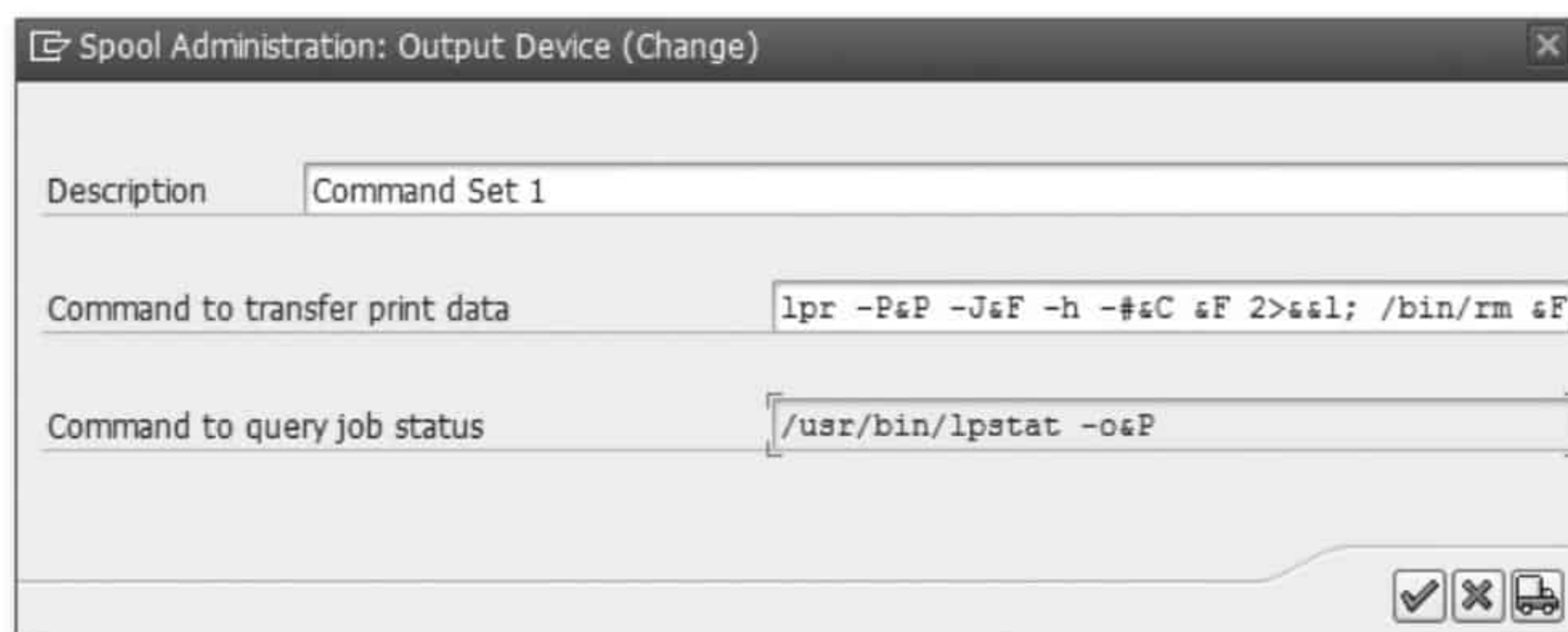
Figure 2.34 Command Set Definition
