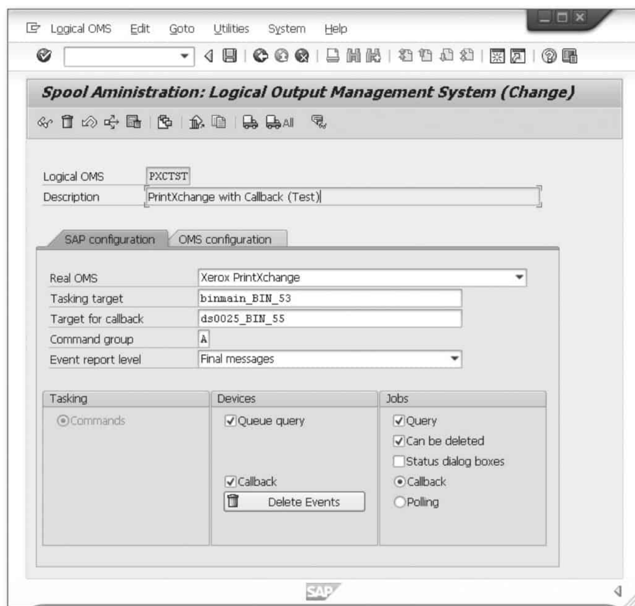
Figure 2.6 LOMS Configuration with Command Groups
