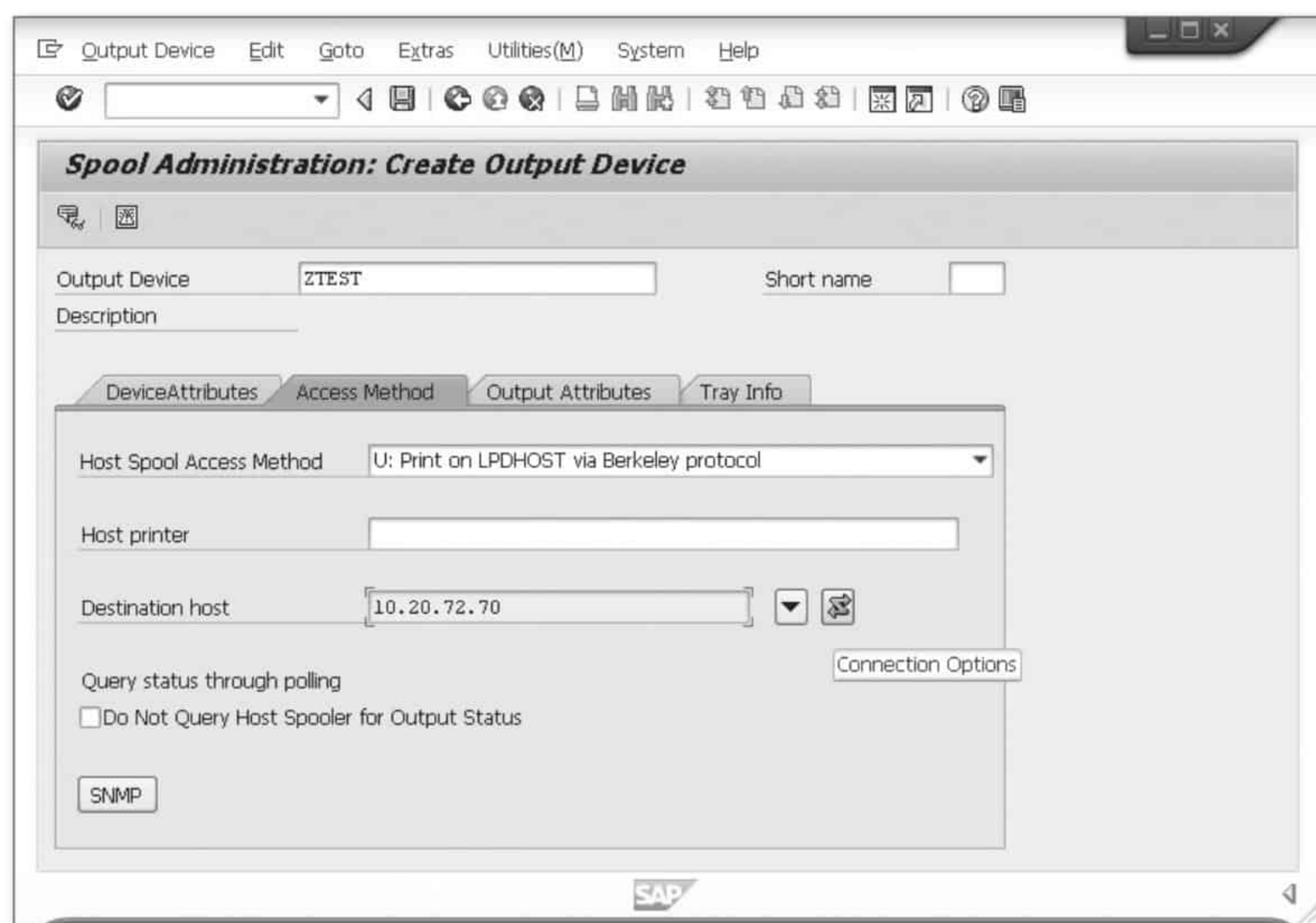
Figure 2.45 Network Print—Access Method
