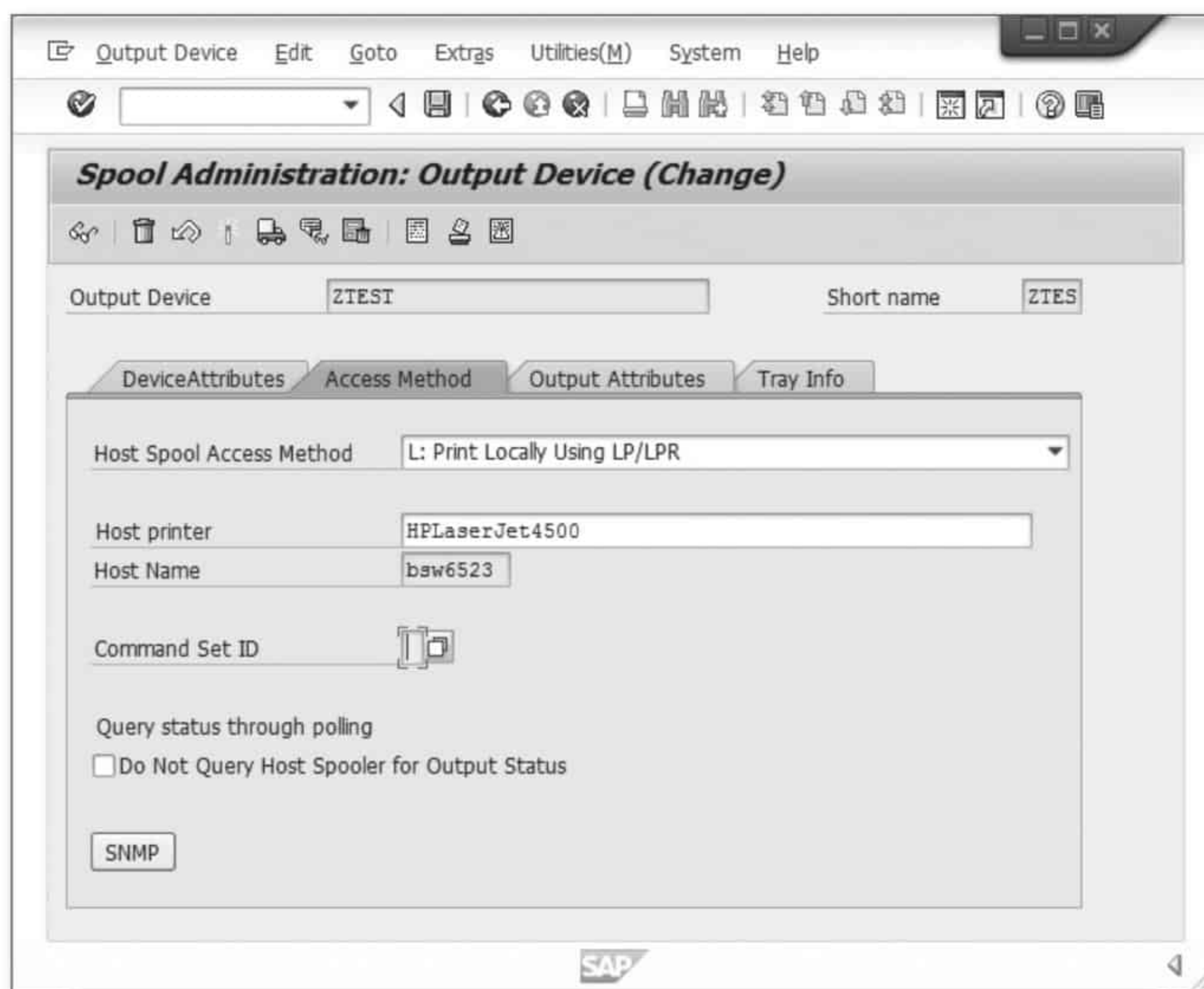
Figure 2.33 Displayed Command Set ID
