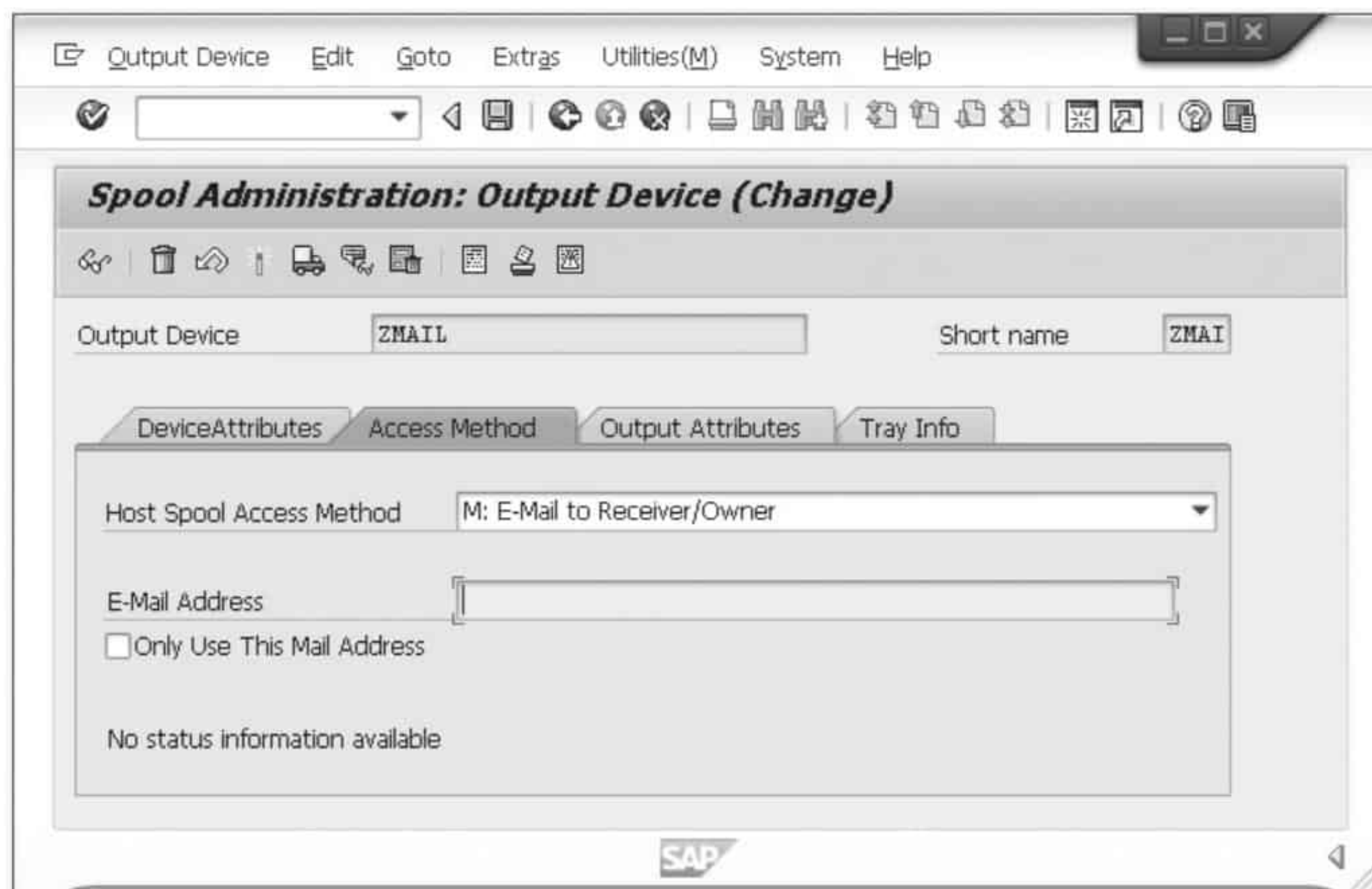
Figure 2.37 Printing via Email—Access Method
