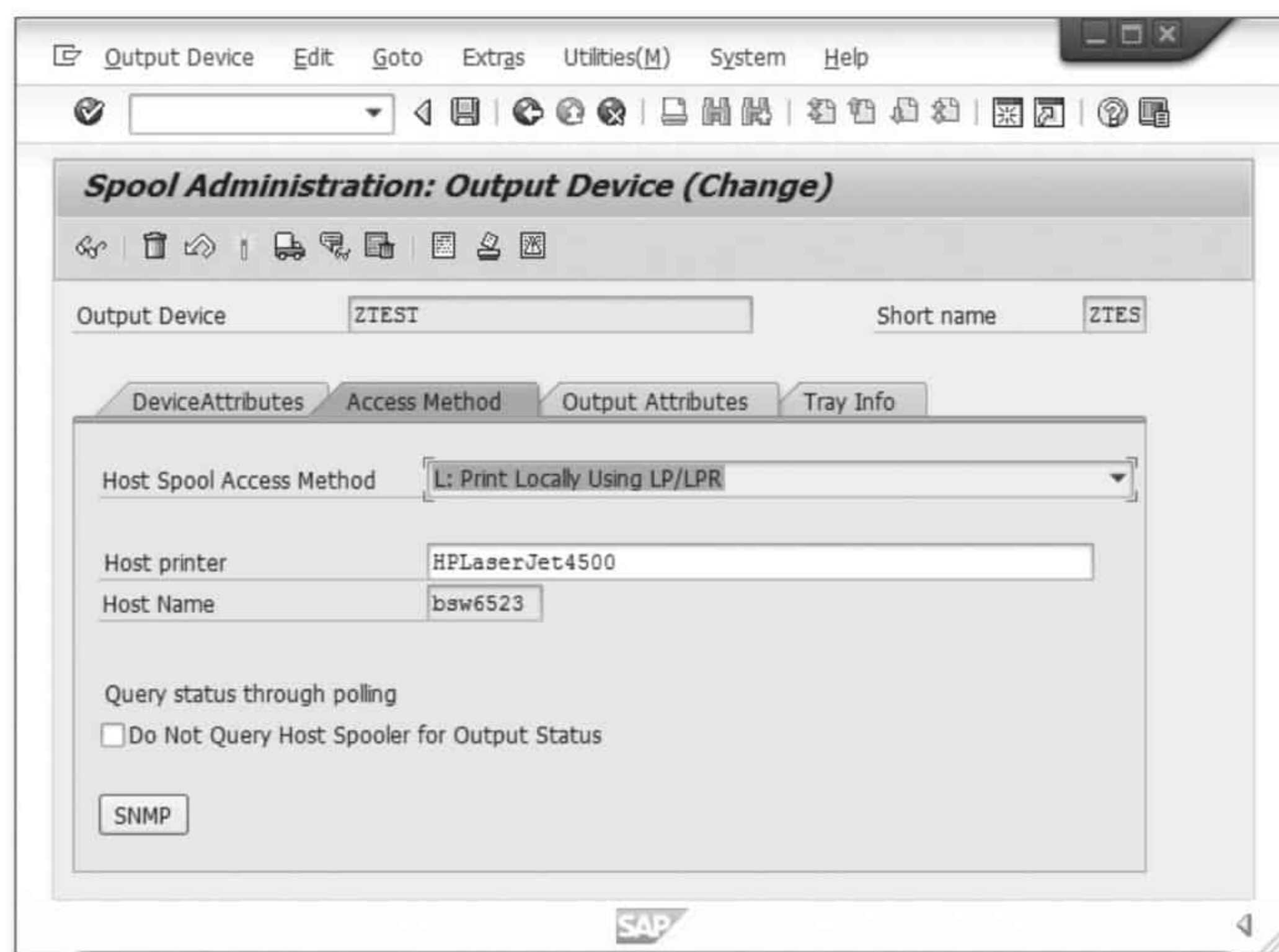
Figure 2.31 Printing via Command Sets—Access Method
