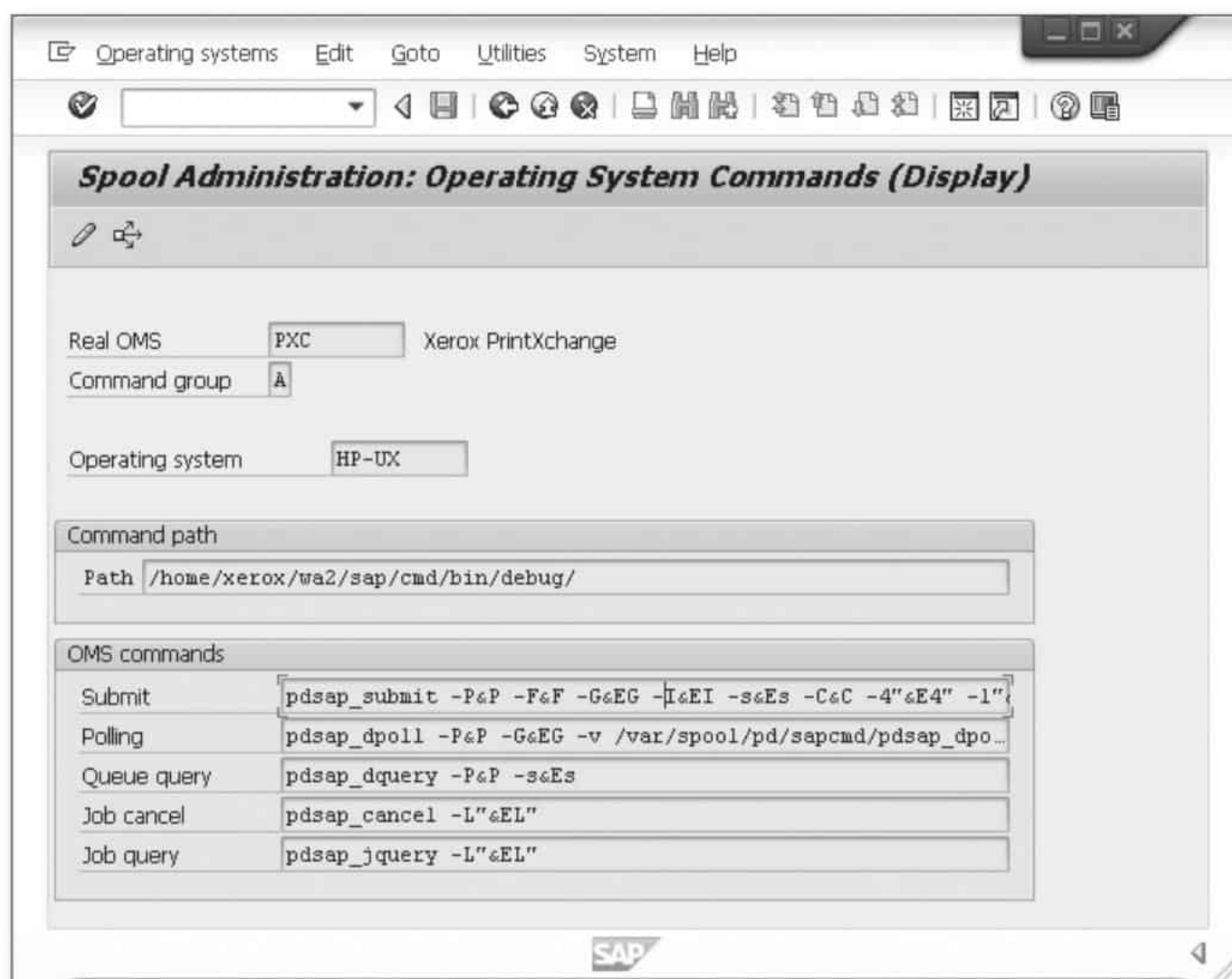
Figure 2.10 OMS Command Group
