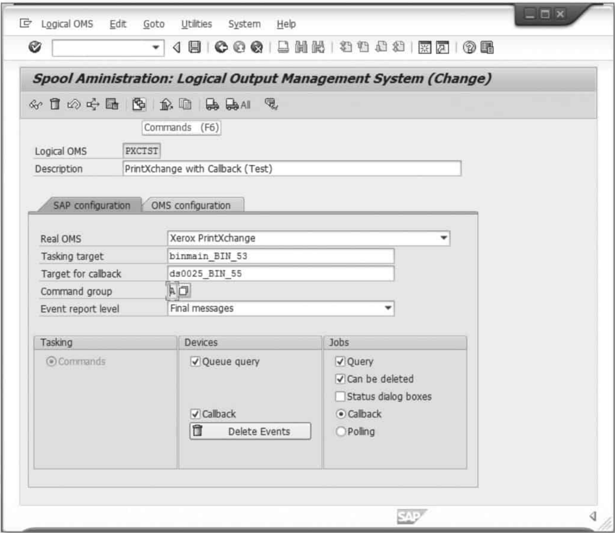
Figure 2.8 Definition of a Command Group
