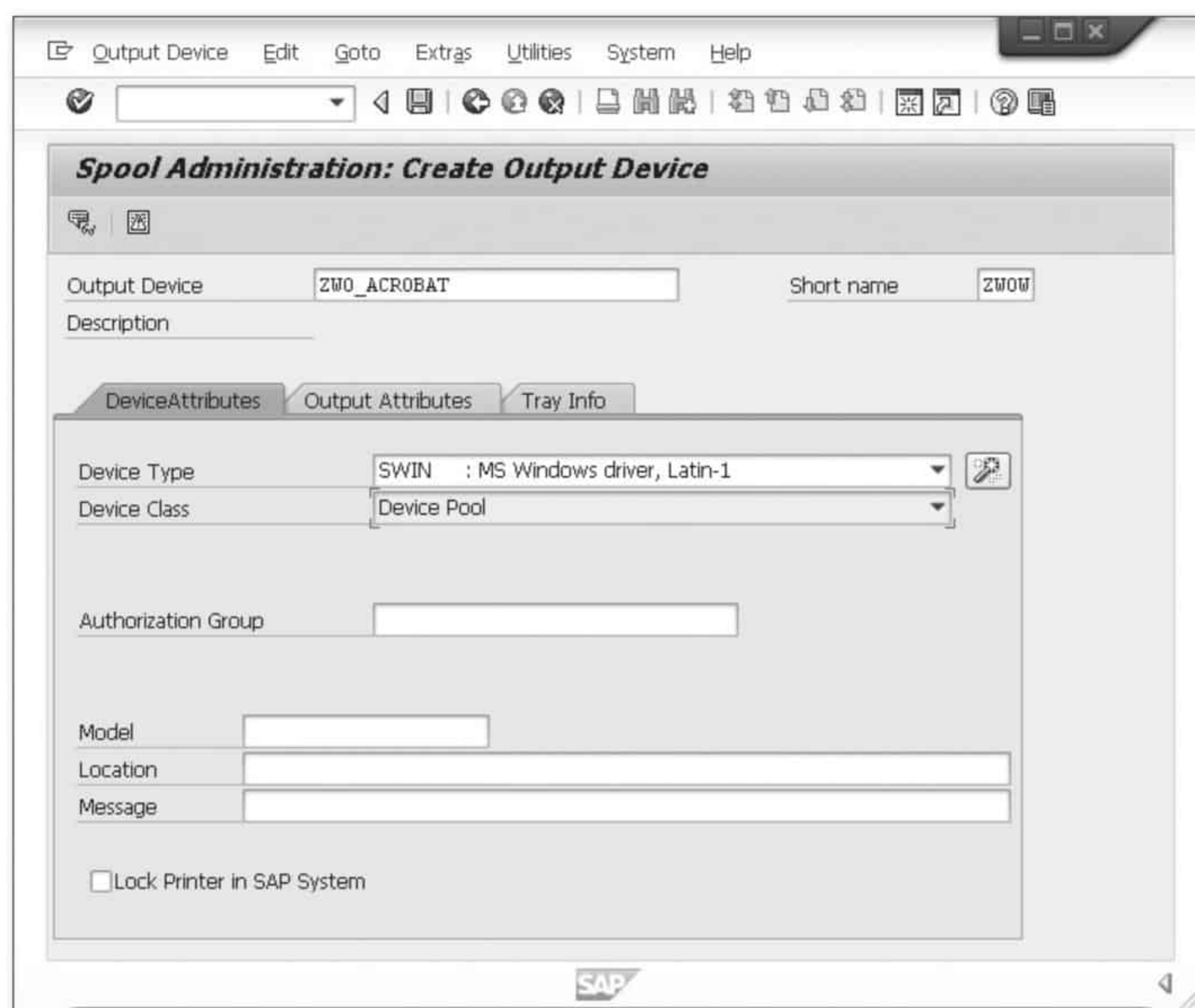
Figure 2.42 Access Method P—DeviceAttributes
