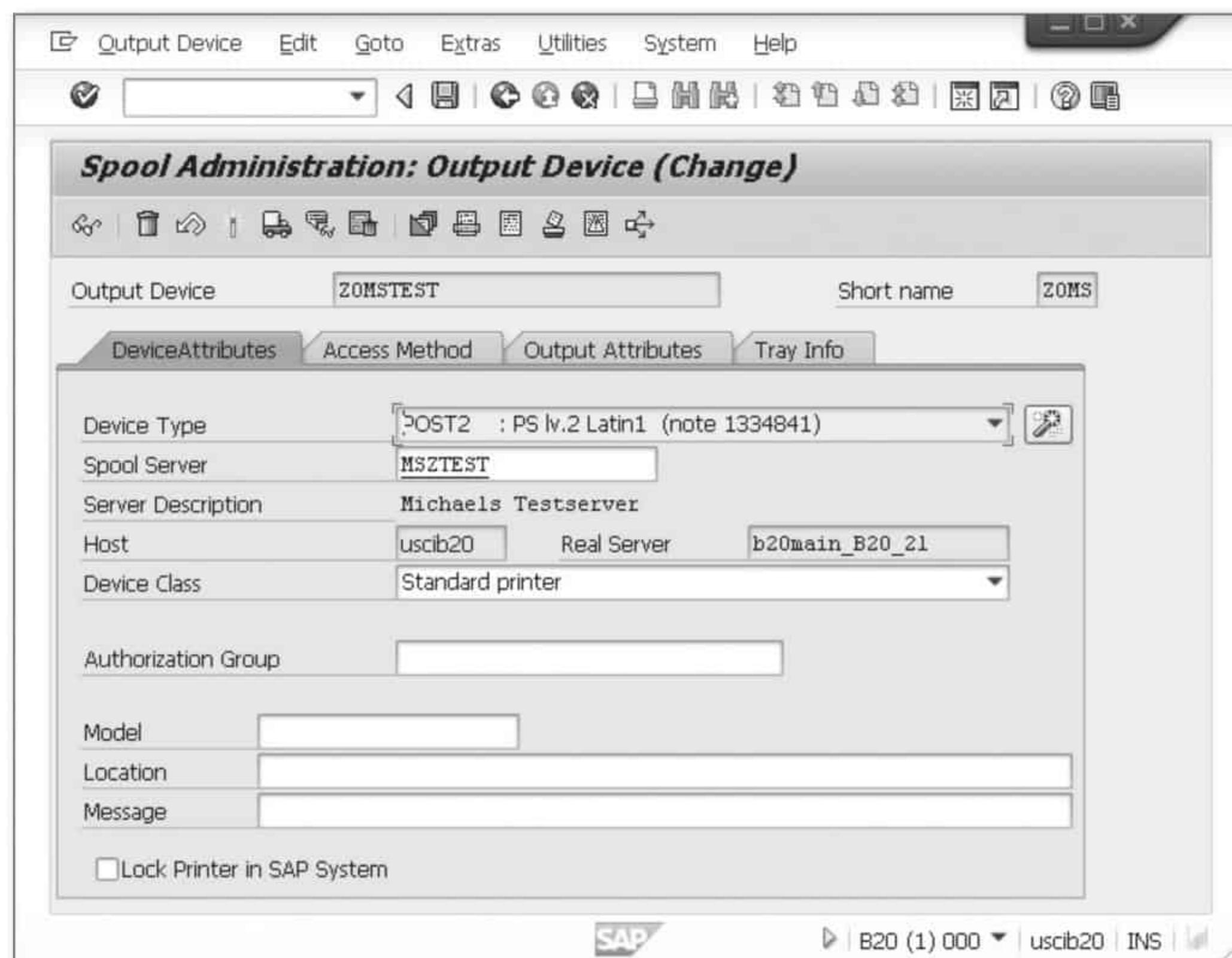
Figure 2.12 Access Method E—DeviceAttributes
