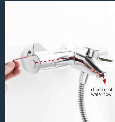
A4128AA Contour 21 Wall mounted thermostatic bath/shower mixer, with lever handles. A unique thermal disinfection facility helps to reduce the risk of bacteria infection (above).
