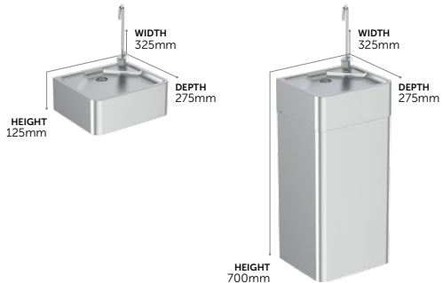
Purita Wall Mounted Drinking Fountains
