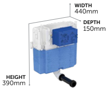
150 Depth Concealed Cistern
