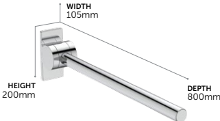
Screw To Wall 80cm Hinged Support Arm
