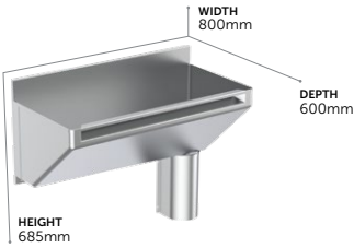
Firth Scrub-up Troughm, 80 cm
