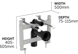
Half Frame for Wall Hung Pans
