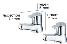
SL Bath Pillar Taps
