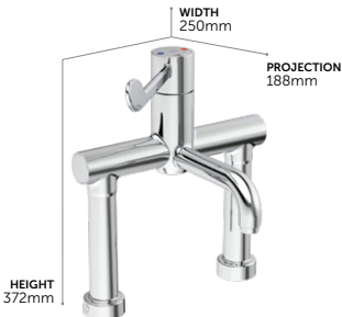
Comfort SQ Deck Mounted Pressure Manual Presure Balance Valve (PBV) Manual Mixer
