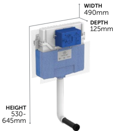
120 Depth WC Concealed Cistern
