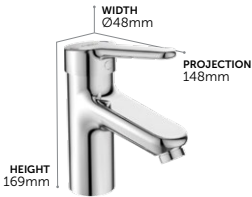
SL Basin Mixer with Level
