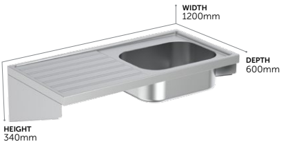
Doon Single Bowl Single Drainer Sinks
