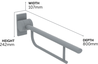
Screw To Wall 80cm Hinged Support Arm G4
