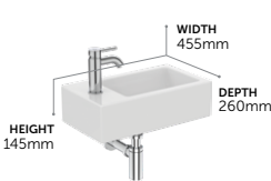
Edit S 45cm Handrinse Basin
