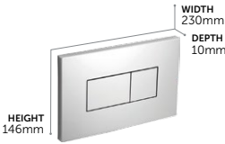
Karisma Dual Flushplate
