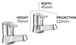
SL Basin Pillar Taps
