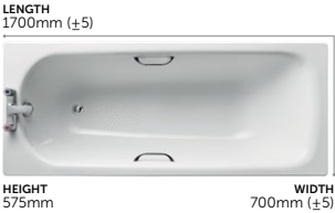
170 x 70cm Standard Gauge Steel Bath
