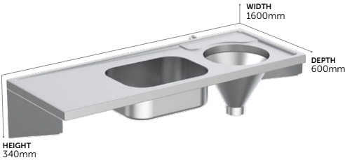
Dee Slop Hoppers with Sink
