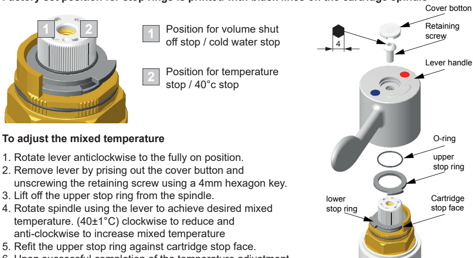
Figure 10.1 Adjusting the pre-set temperature
