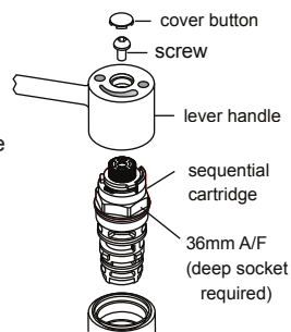
Figure 10.2 Exploded view showing sequential cartridge
