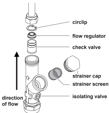
Fig.11.2 Exploded view of isolating valve
