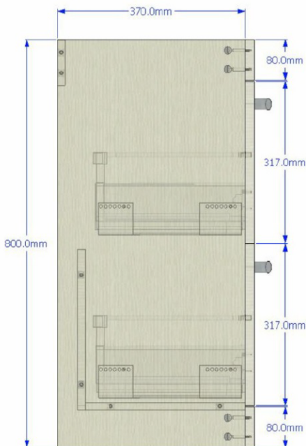
Left Elevation
