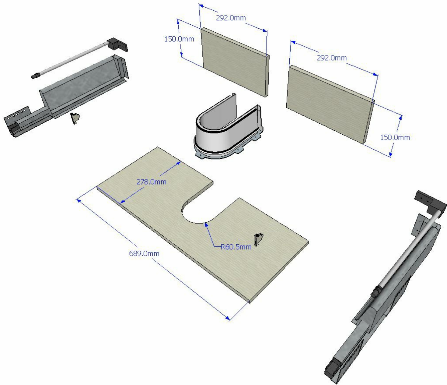
Top Drawer - Exploded View
