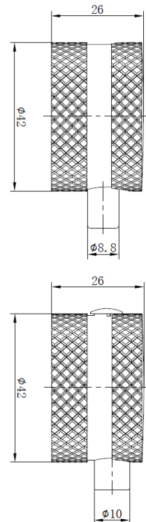
Dimensions (Measurements in mm)
