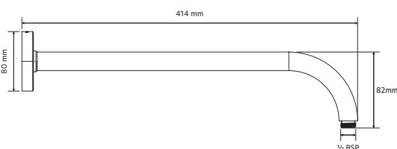
Wall Arm
