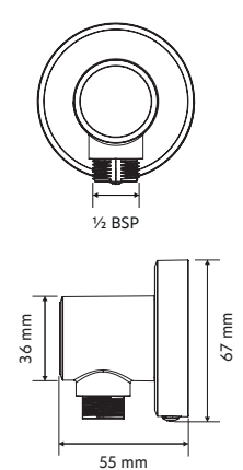
Wall Outlet
