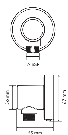
Wall Outlet
