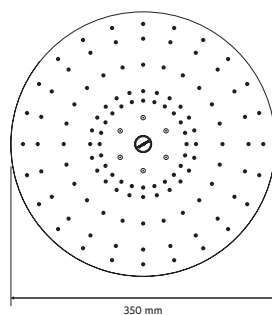
350mm Drencher
