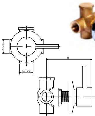
sola shower diverter
