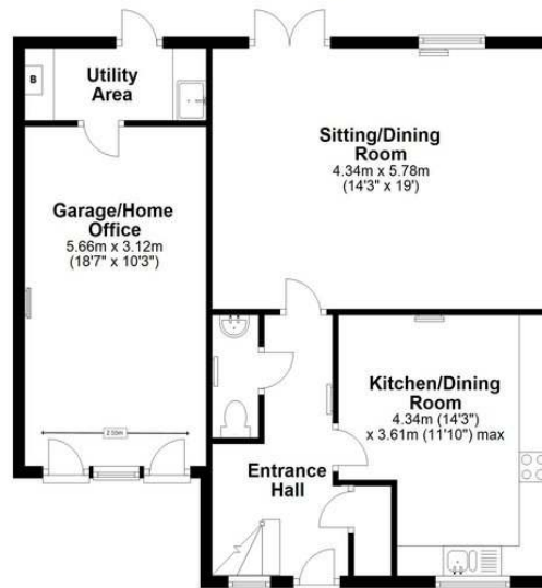
Ground Floor Approx. 80.5 sq. metres (866.5 sq. feet)
