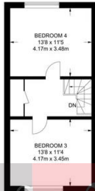
SECOND FLOOR 396 SQ FT / 36.8 SQ M
