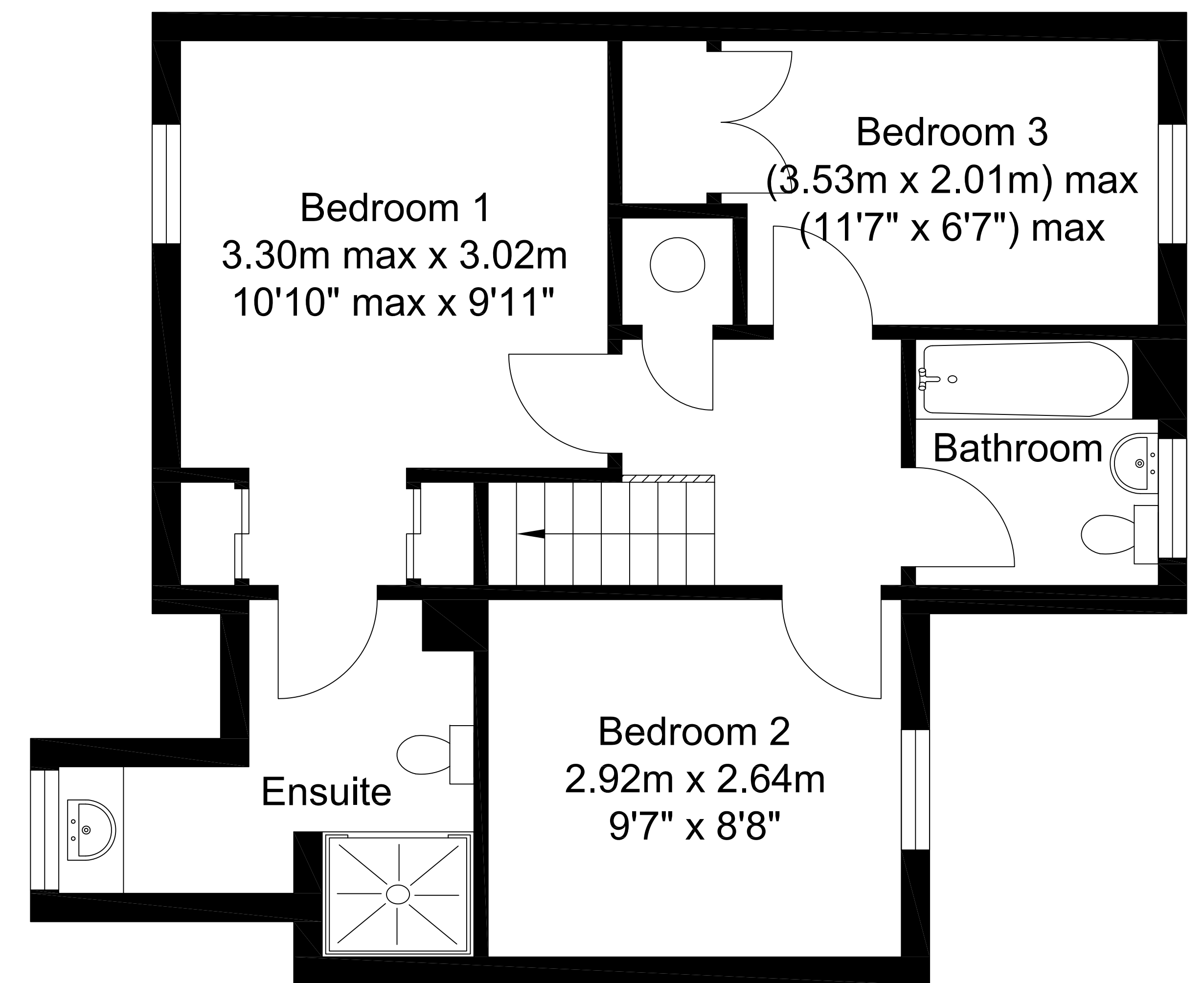
First Floor Total Approximate Area 458.65 sq. ft. (42.61 sq. m)
