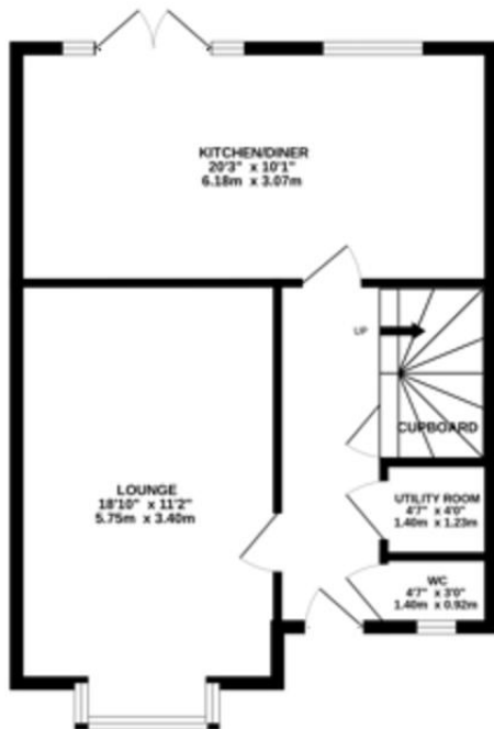
GROUND FLOOR 539 sq.ft. (50.1 sq.m.) approx.
