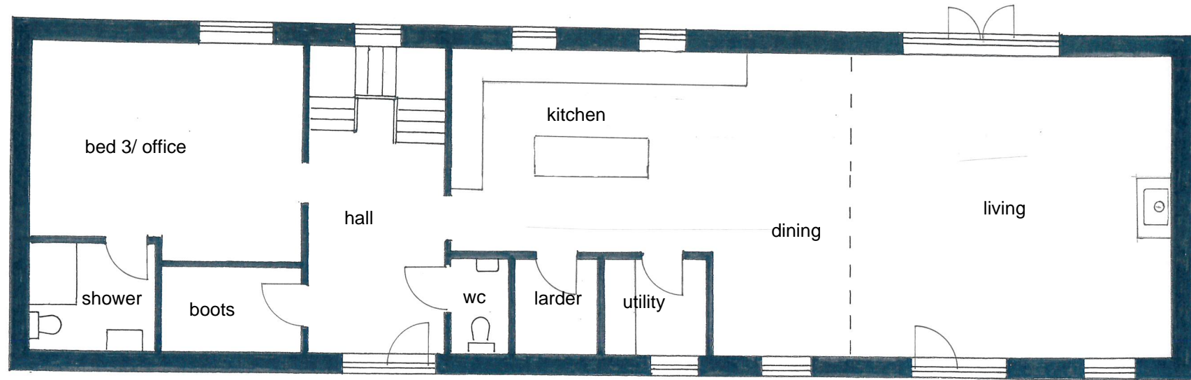
ground floor
