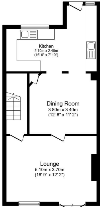
Ground Floor Floor area 51.7 sq.m. (556 sq.ft.)
