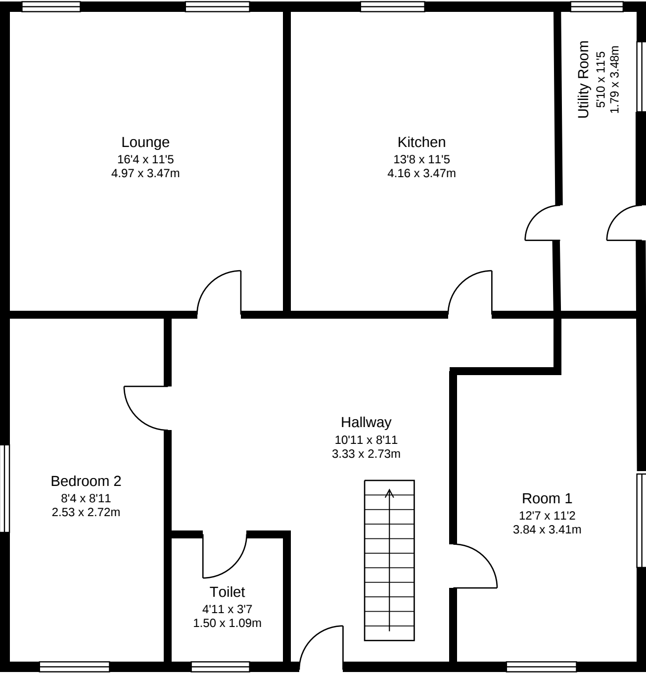
Ground Floor
