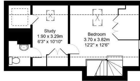
Second Floor Area: 24.1 m 2 ... 259 ft 2
