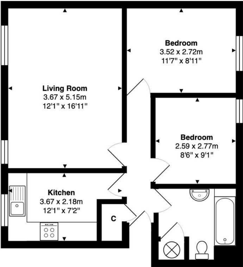
First Floor Approximate Gross Internal Area 55.9 m 2 ... 602 ft 2
