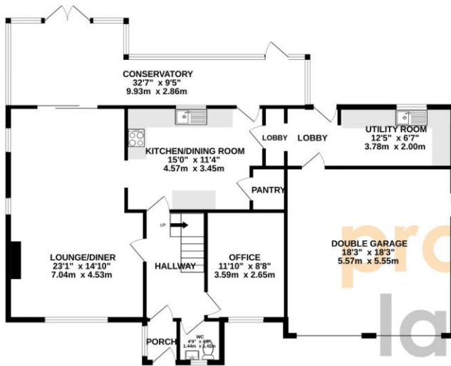
GROUND FLOOR 1413 sq.ft. (131.2 sq.m.) approx.
