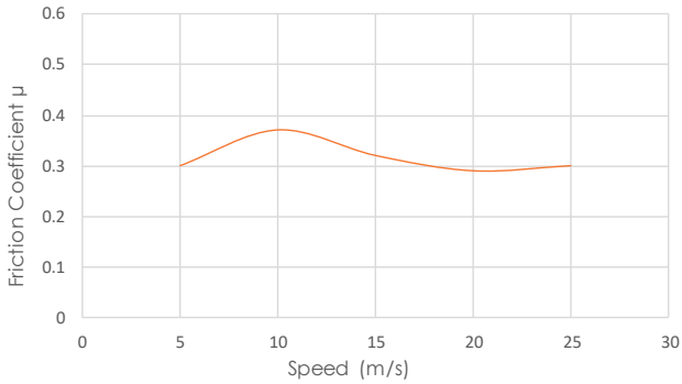
Speed Sensitivity
