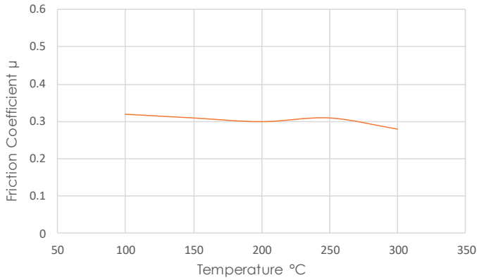
Temperature Sensitivity
