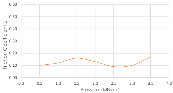
Pressure Sensitivity
