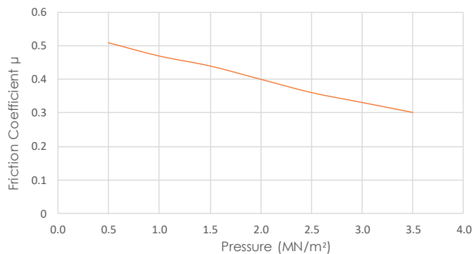
Pressure Sensitivity
