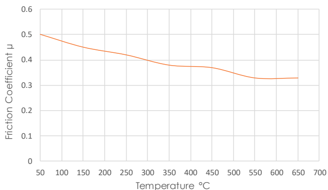
Temperature Sensitivity
