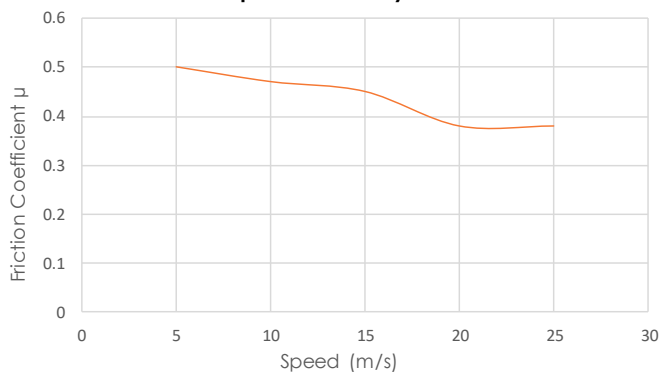
Speed Sensitivity
