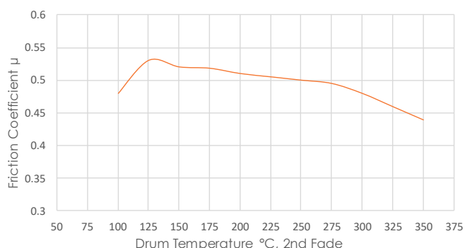
Friction Coefficient
