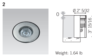
AISI 316L stainless steel round flush trim
