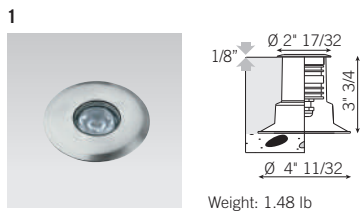
AISI 316L stainless steel round trim
