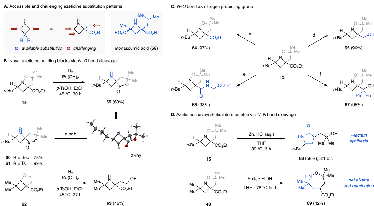
Fig 4. Synthetic modification of azetidine products. A. Currently available azetidine building blocks and azetidine-containing natural products B. Hydrogenolysis provides access to unprotected azetidines C. The N -O bond in the azetidine products is tolerant of multiple synthetic transformations D. Azetidines can undergo C - N cleavage reactions. Conditions: a) \text{Boc}_2\text{O} , DMAP, \text{CH}_2\text{Cl}_2 , rt; (for 60 ) b) p\text{-TsCl} , \text{K}_2\text{CO}_3 , MeCN, 80 °C (for 61 ) c) \text{LiOH} , \text{H}_2\text{O} , MeOH, rt; then, glycine ethyl ester·HCl, DMAP, EDC·HCl, \text{CH}_2\text{Cl}_2 , rt f) \text{PhMgBr} , THF, 0 °C.
