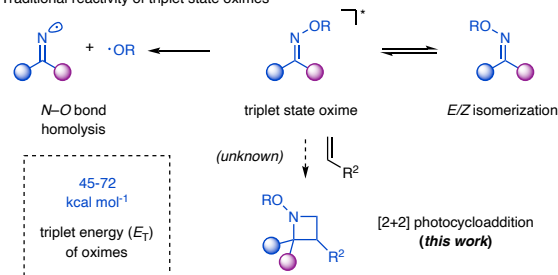
C. Intermolecular aza Paternò-Büchi reaction via triplet state oximes (this work)
