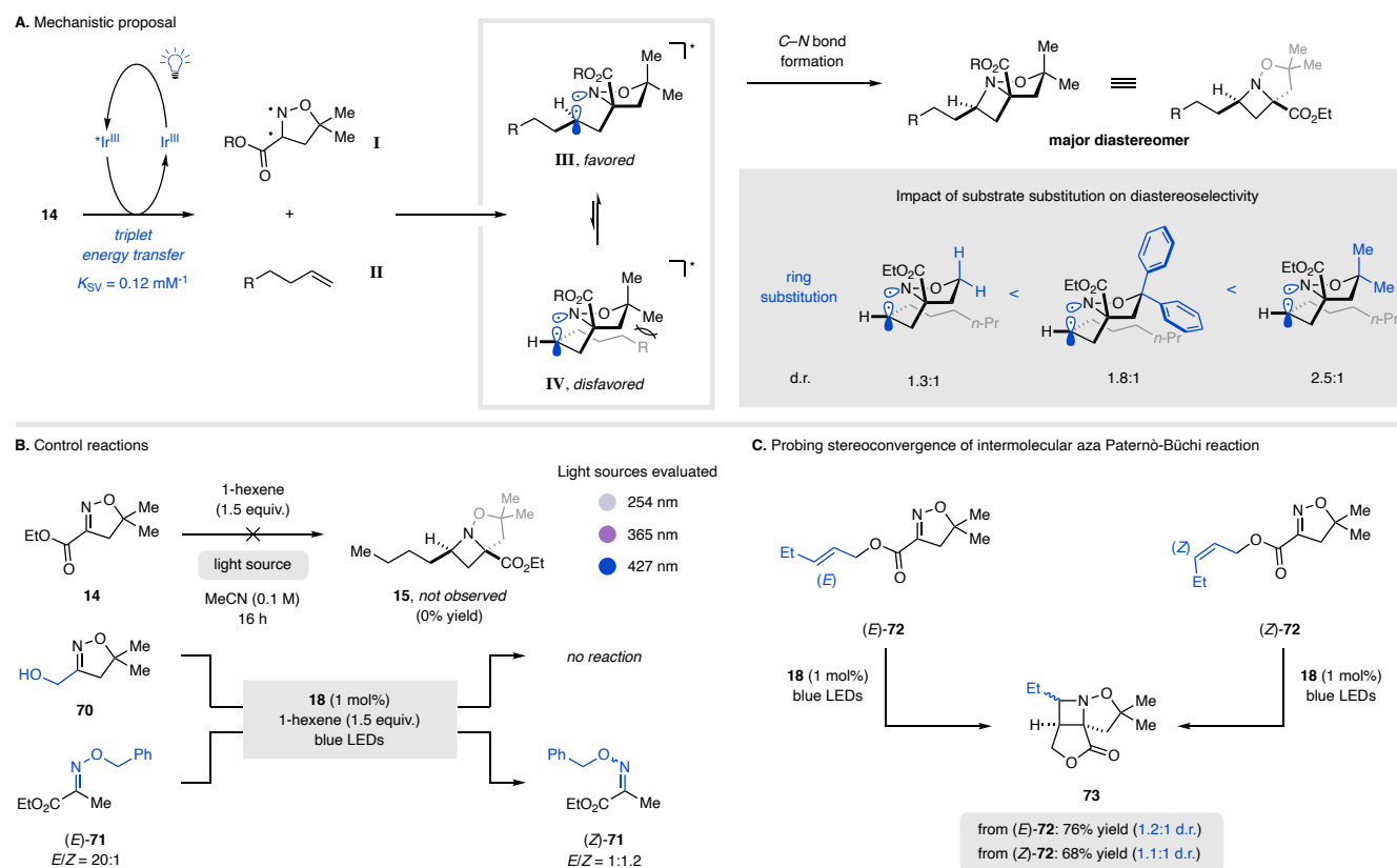
Fig 5. Mechanistic investigation of the title reaction A. Mechanistic proposal relying on a triplet state oxime B. Control reactions C. Probing stereoconvergence of the title reaction. K_{\text{SV}} = Stern-Volmer quenching constant
