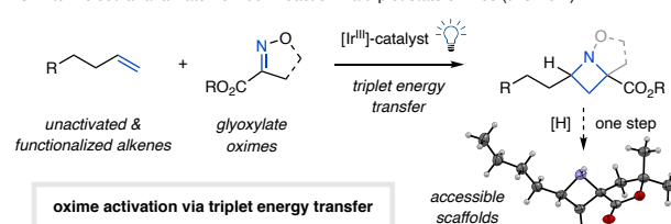
C. Intermolecular aza Paternò-Büchi reaction via triplet state oximes (this work)
