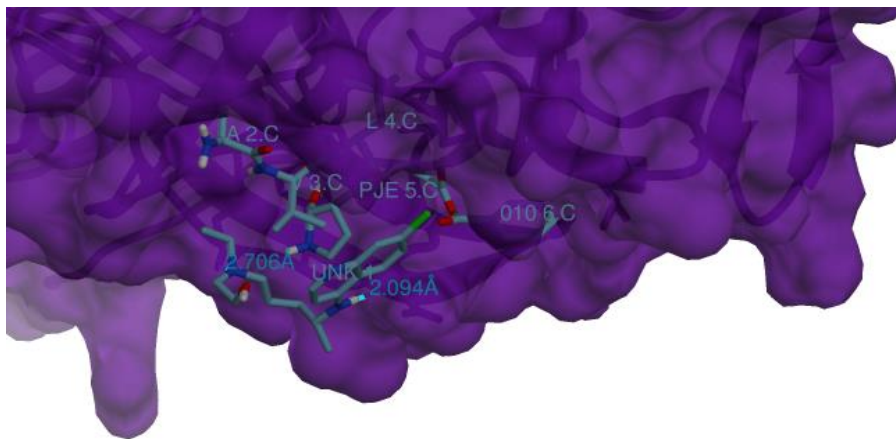
Figure 6: Hychloroquincomplex2 interactions with 6LU7
