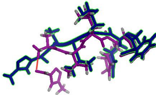
Figure 4: superimposing result for orientation of the ligands, the original structure is in blue, the re-docked complex is in magenta.
