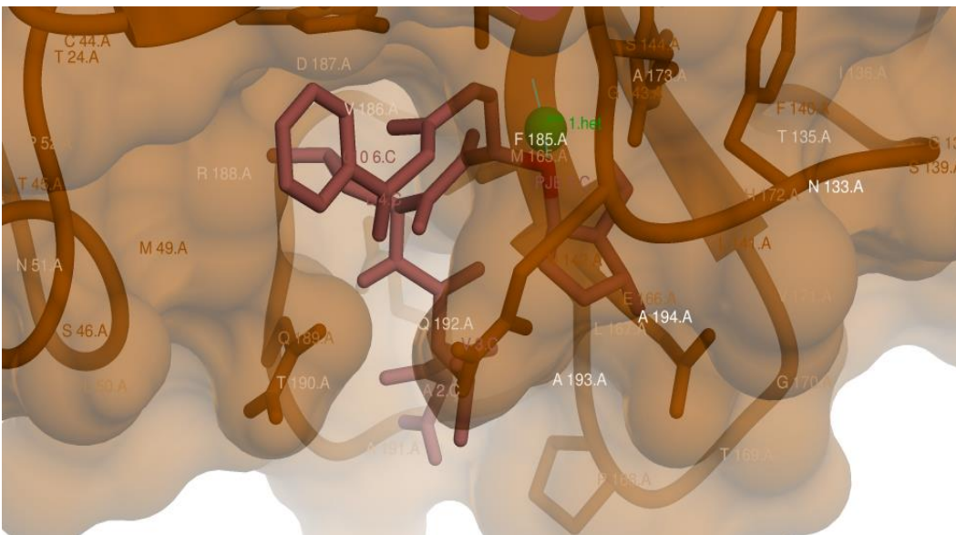
Figure 9:zinc clathes with 6LU7
