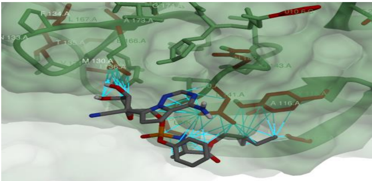
Figure 15: Remdisvir's complex 7 interactions in the binding site of 6LU7
