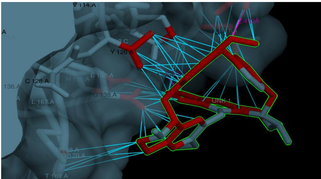
Figure 11:cephranthine complex2 interactions with 6LU7 binding site
