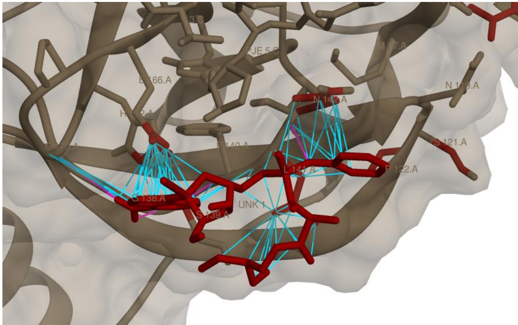
Figure 12: Remdisvir's complex 1 interactions in the binding site of 6LU7
