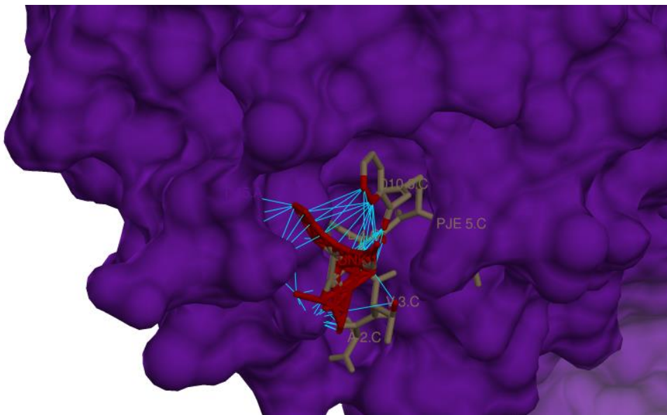
Figure 7:AZITHROMYCIN complex1 interactions with 6LU7
