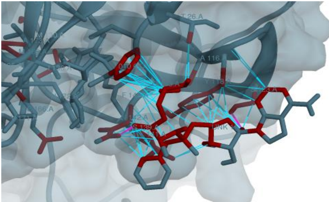
Figure 13: Remdisvir's complex 2 interactions in the binding site of 6LU7
