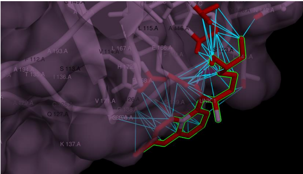
Figure 8:chloroquin WanderVlas interactions with 6LU7
