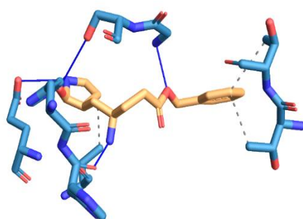
Figure 1 : Chemical structure for potential drugs treat COVID-19 (23)
