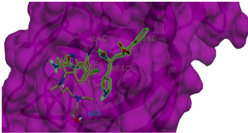
Figure 5:hydroxychloroquincomplex1 interactions with 6LU7
