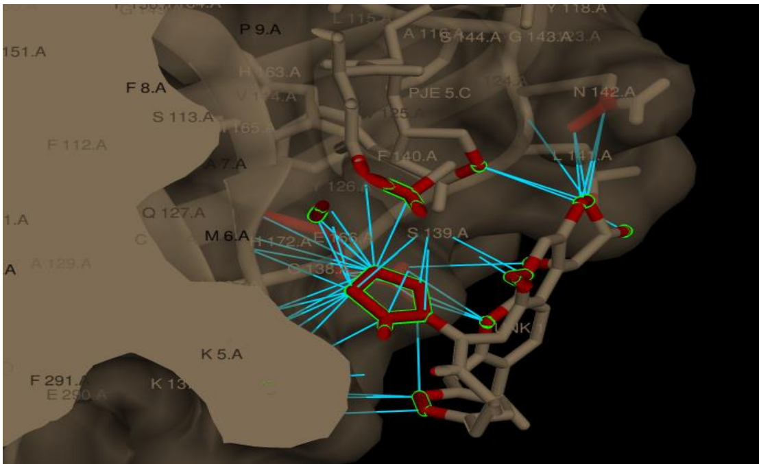
Figure 10:cephranthine complex1 interactions with 6LU7 binding site
