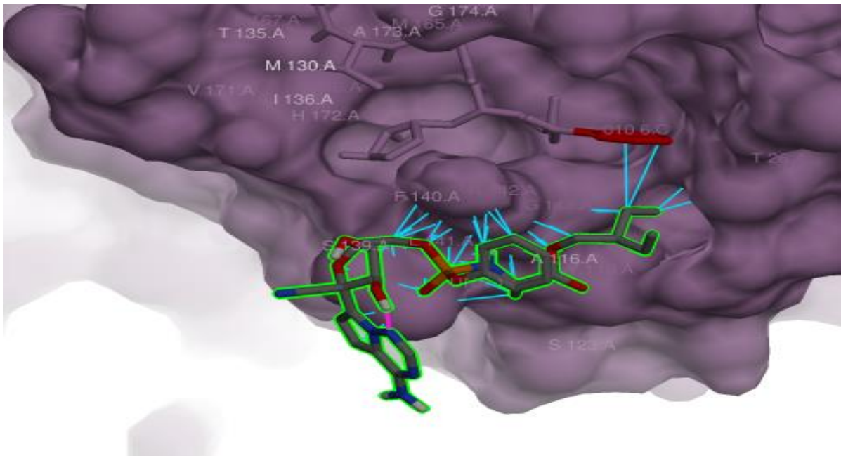
Figure 14: Remdisvir's complex 3 interactions in the binding site of 6LU7
