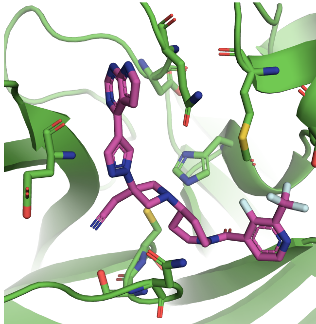
Figure A3: Docking pose of Itacitinib in 3CL protease active site. Non-covalent docking predicted the binding affinity to be -8.3 kcal/mol.
