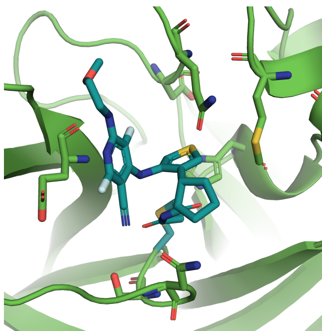
Figure A9: Covalent docking pose of BEN-VAN-d2b-11 in 3CL protease active site. Covalent docking predicted the binding affinity to be -2.2 kcal/mol.
