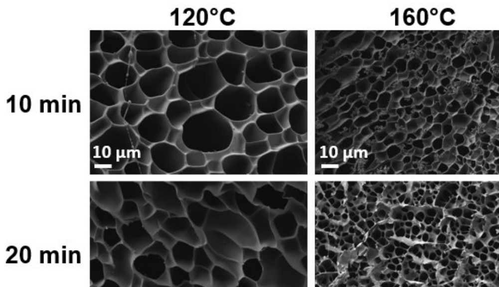
Figure 7. SEM micrographs at 2kV EHT of the PEOx/P[PM-co-MA] blends after heat treatment at different temperature and time. All PEOx/P[PM-co-MA] samples were obtained after incubation for 40 min with 20 wt. % of polyperoxide.
