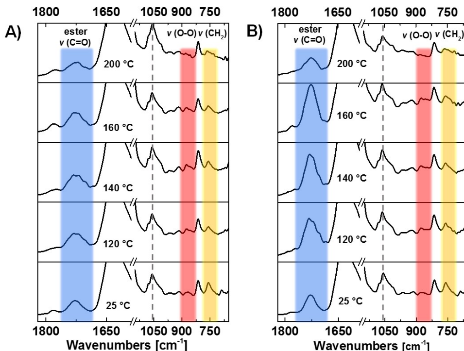
Figure 5. FTIR spectra of the (crosslinked) PETox with 20 wt. % of P[PM-co-MA] (A) and P[PM-co-BA-co-MA] (B) crosslinked at different temperatures and 40 min of crosslinking time.
