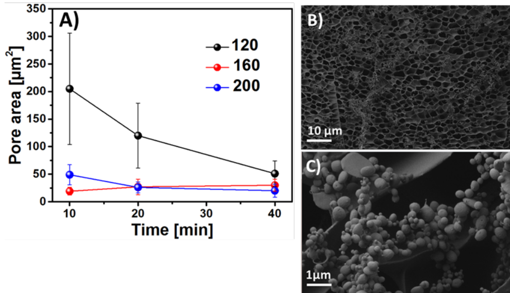
Figure 8. A) - Impact of crosslinking temperature and incubation time on pore area; B), C) - Appearance of the agglomerates obtained during the heating process. EHT: 2kV.
