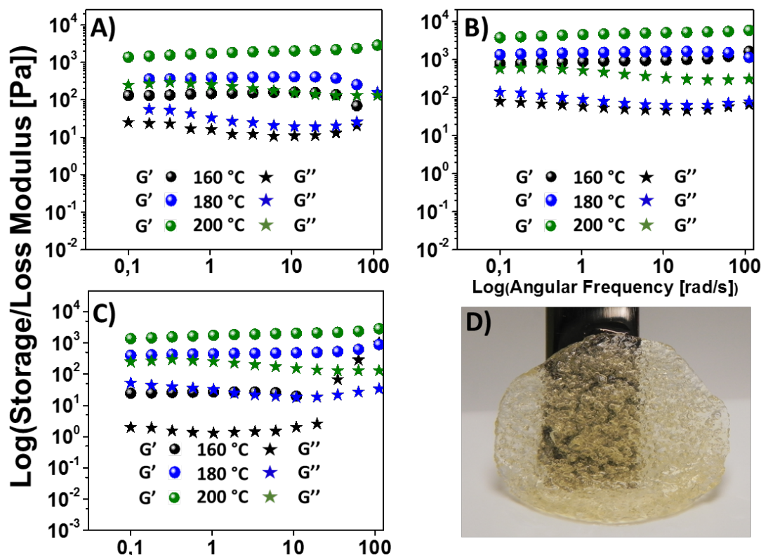
Figure 13. Frequency sweep of PETox/polyperoxide based hydrogels obtained after incubation for 40 min at different crosslinking temperatures (160 – 200 °C) and different concentration of peroxide containing copolymer crosslinker: A) P[PM-co-MA] 15 wt. %; B) P[PM-co-MA] 20 wt. % C) P[PM-co-BA-co-MA] 15 wt.%. D) Visual appearance of hydrogel, obtained at 160 °C after 40 min using P[PM-co-MA] at 20 wt. %.
