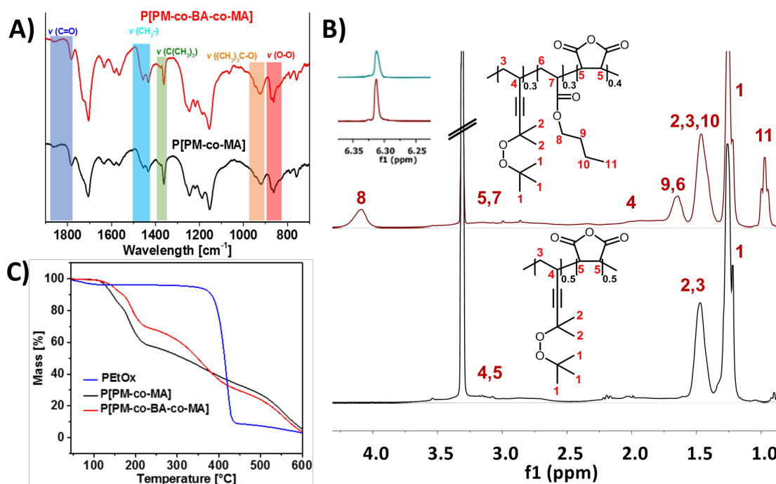
Figure 2. Characterization of the peroxide copolymers. A) FTIR spectra of the P[PM-co-MA] and P[PM-co-BA-co-MA] respectively; B) ^1\text{H} NMR spectra of the P[PM-co-BA-co-MA] (red) and P[PM-co-MA] (black), respectively; C) Thermogravimetric analysis of the used polymers of employed polyperoxides and commercial poly(2-ethyl-2-oxazoline) (Aquazol® 500).
