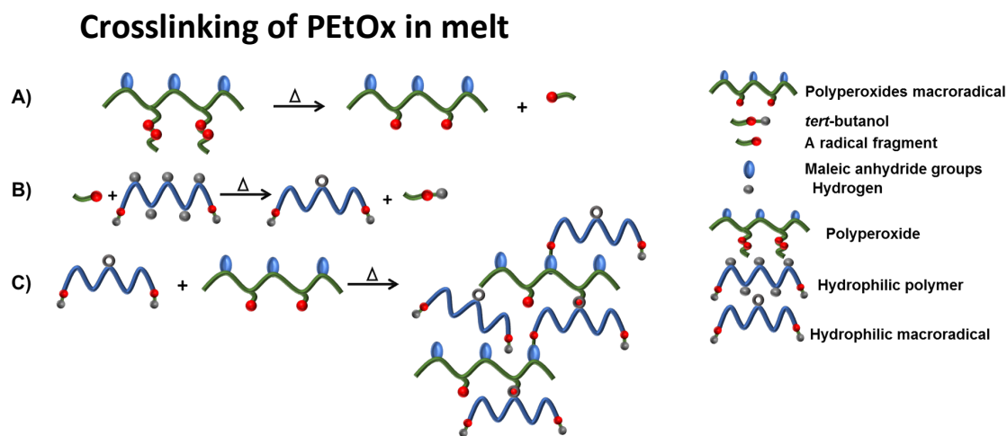
Figure 4. Simplified schematic illustration of peroxide containing copolymer induced cross-linking: A) thermal decomposition of peroxide copolymer into two radicals when exposed to heat followed by B) hydrogen abstraction from polymer chain by primary radical and C) recombination reaction of polymer radicals.
