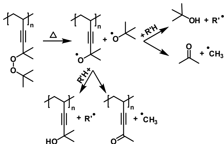
Figure 3. Schematic illustration of the thermal decomposition of peroxide groups in peroxide containing copolymer.
