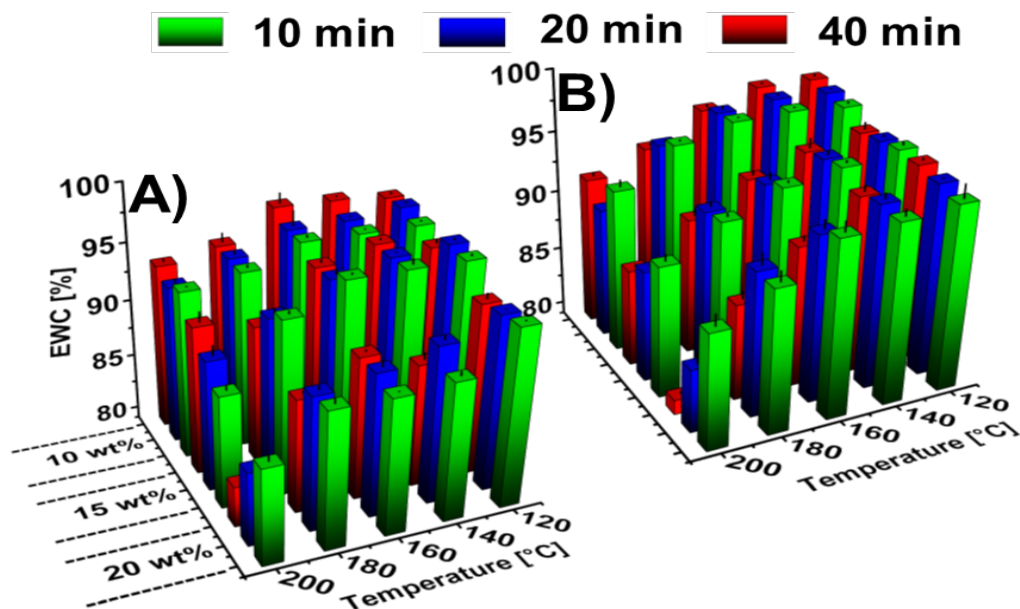
Figure 10. Influence of the peroxide containing copolymer concentration (10 - 20 wt.%), temperature (120-200 °C) and crosslinking time 10 – 40 min, on the equilibrium water content (EWC) of P[EtOx] hydrogels. A) - P[PM-co-MA] and B) - P[PM-co-BA-co-MA].
