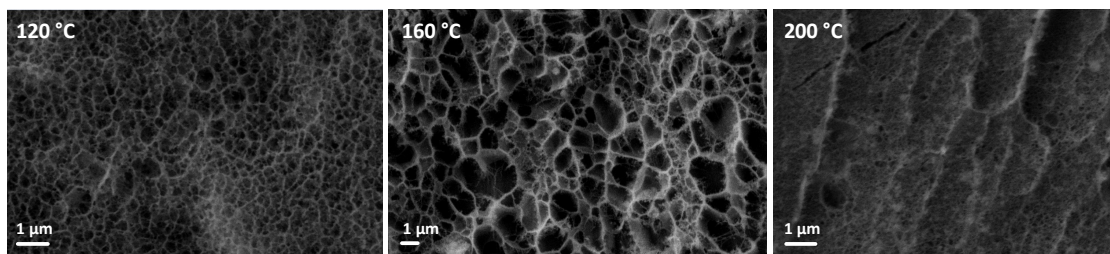
Figure 9. Cryo-SEM analysis (EHT: 8kV) of the samples obtained after 40 min of treatment at different temperature. The concentration of P[PM-co-MA] is 20 wt.%.
