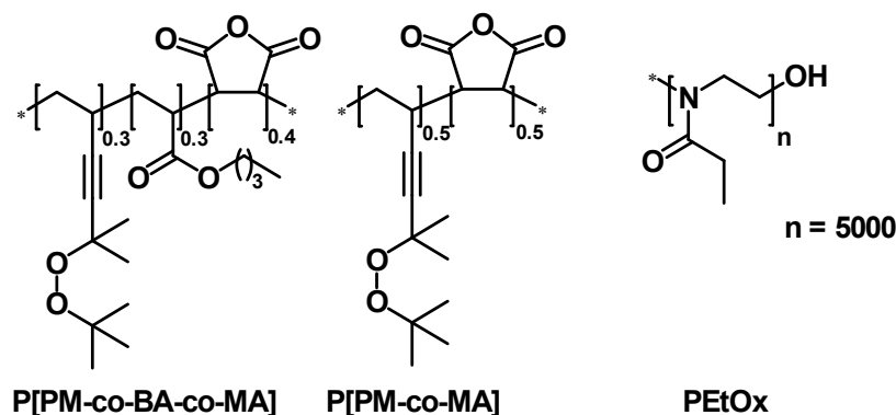
Figure 1. Schematic illustration of the chemical structure of the used polymers. P[PM-co-BA-co-MA] – poly(5-tert-butylperoxy-5-methyl-1-hexen-3-yne-co-butyl acrylate-co-maleic anhydride); P[PM-co-MA] – poly(5-tert-butylperoxy-5-methyl-1-hexen-3-yne-co-maleic anhydride); PEtOx – poly(2-ethyl-2-oxazoline)
