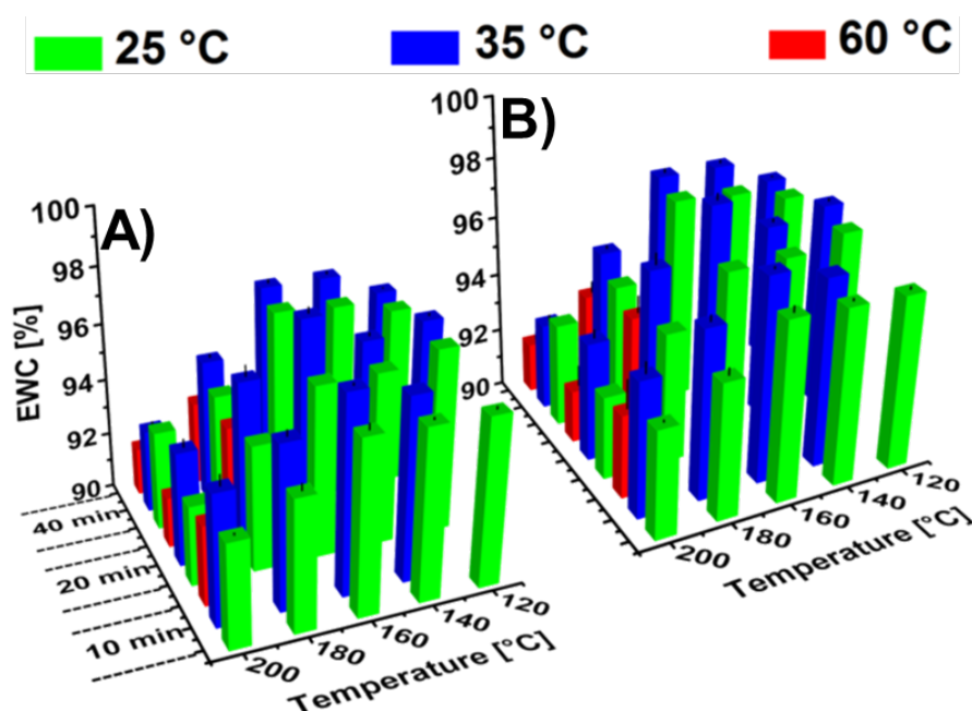
Figure 11. Dependence of the swelling behavior on the temperature of swelling process. Hydrogels were obtained with the concentration of P[PM-co-MA] A) - 10 wt. % and B) – 15 wt. %.
