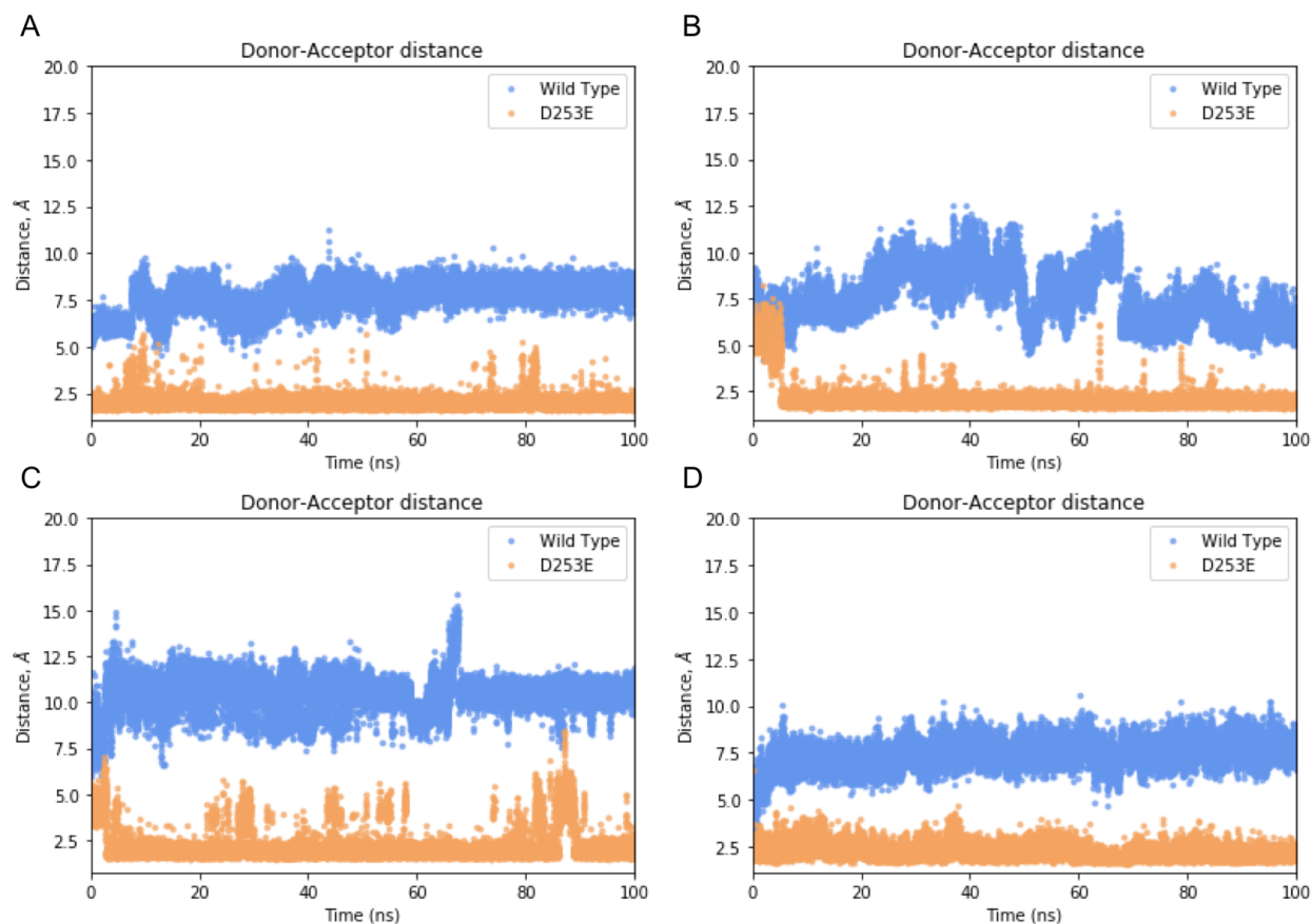
Figure S1. The donor-acceptor distances found during 100 ns of MD simulation in Wild Type OPH complexed to paraoxon and the mutant D253E complexed to paraoxon between: A) Thr 54 and His 55, B) His 57 and Trp 302, C) Thr 200 and His 201, and D) Leu 271 and His 254. We found that, during the simulations on the OPH variant (D253E) complex, the distances between : i) Thr 54 and His 55, ii) His 57 and Trp 302, iii) Thr 200 and His 201, and Leu 271 and His 254 are short (fluctuating around 2 Å), signaling the formation of hydrogen bonds between the residues belonging to each of these pairs. The respective donor-acceptor distances during MD simulation on the WT complex are greater than the typical distance of a hydrogen bond (2 Å). These results show that the mutation D253E induced four different hydrogen bonds near the active site of OPH.
