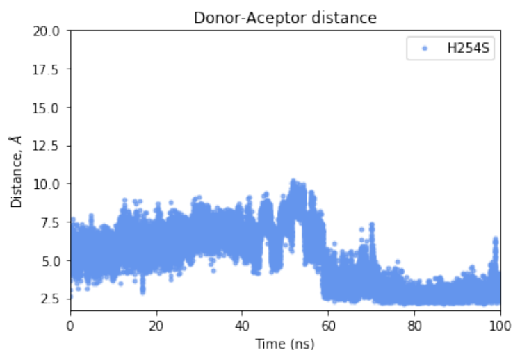
Figure S4. The donor-acceptor distance found during 100 ns of MD simulation on OPH:H254S between a crystal water molecule and the mutated residue H254S. After 60 ns of MD on the mutant complex (H254S), a water molecule belonging to the active site of OPH and involved in the coordination of Zn(II) establishes a hydrogen bond with Ser 254 with a distance fluctuating around 2.5 Å.
