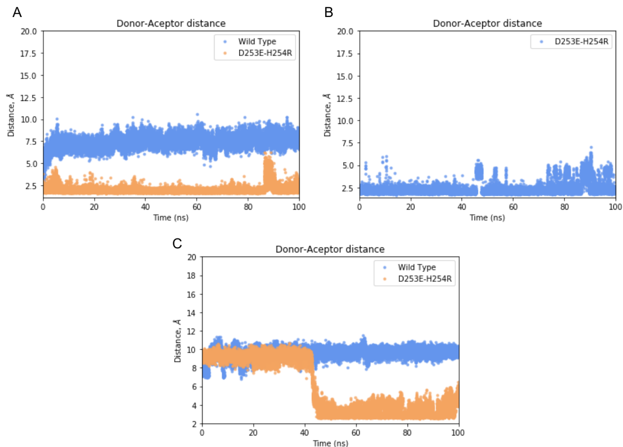
Figure S2. The donor-acceptor distances found during 100 ns of MD simulation on WT OPH complexed to paraoxon and the double mutant D253E-H254R complexed to paraoxon between: A) The residue at position 254 (His in WT OPH and Arg in the double mutant) and Leu 271, Arg 254 and His 257, and Asp 100 and Lys 169. We found that during the simulations on the double mutant (D253E-H254R) complex, the distances between: i) H/R 254 and Leu 271, ii) Arg 254 and His 257, and iii) Asp 100 and Lys 169 are short (fluctuating around 2 Å), signaling the formation of hydrogen bonds between the residues belonging to each of these pairs. The respective donor-acceptor distances during MD simulation on the WT OPH complex are greater than the typical distance of a hydrogen bond (2 Å). The distance between residues Arg 254 and His 257 corresponding to the WT complex are not shown on the plots of this figure since Arg 254 was found far from the residue at position 257 during the respective MD simulations. These results show that the double mutant D253E-H254R induced three different hydrogen bonds near the active site of OPH.
