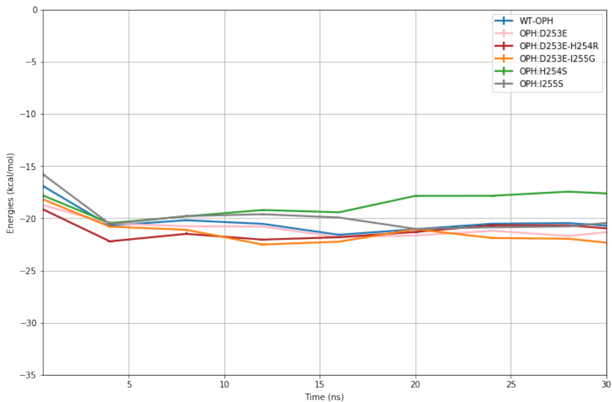
Figure S6. Absolute binding free energy calculations of OPH complexes. The binding free energies of paraoxon complexed with WT-OPH in blue, OPH:D2253E in pink, OPH:D253E-H254R in red, OPH:D253E-I255G in orange, OPH:H254S in green, and OPH:I255S in grey were computed in implicit solvent after 30 ns/thermodynamic state. Overall, the simulations are sufficiently converged and the binding of paraoxon to the mutant forms D253E, D253E-H254R, and D253E-I255G is more favorable than its binding to WT-OPH.
