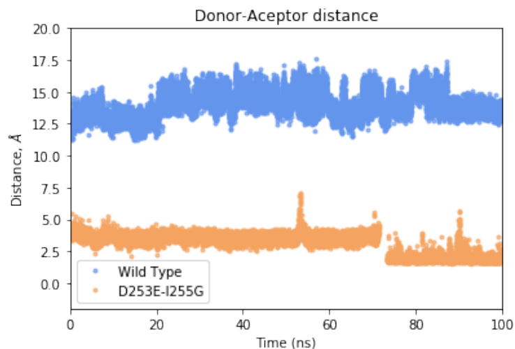
Figure S3. The donor-acceptor distances found during 100 ns of MD simulation on WT OPH:paraoxon complex and the double mutant D253E-I255G complexed to paraoxon between Asp 100 and His 257. These residues do not interact during the simulations of the WT complex. Asp 100 and His 257 are closer during the simulations of the double mutant complex compared to the simulations on the WT complex. Also, these residues come close after 75 of MD on the mutant complex (D253E-I255G), where they establish a stable hydrogen bond with a distance fluctuating around 2 Å.
