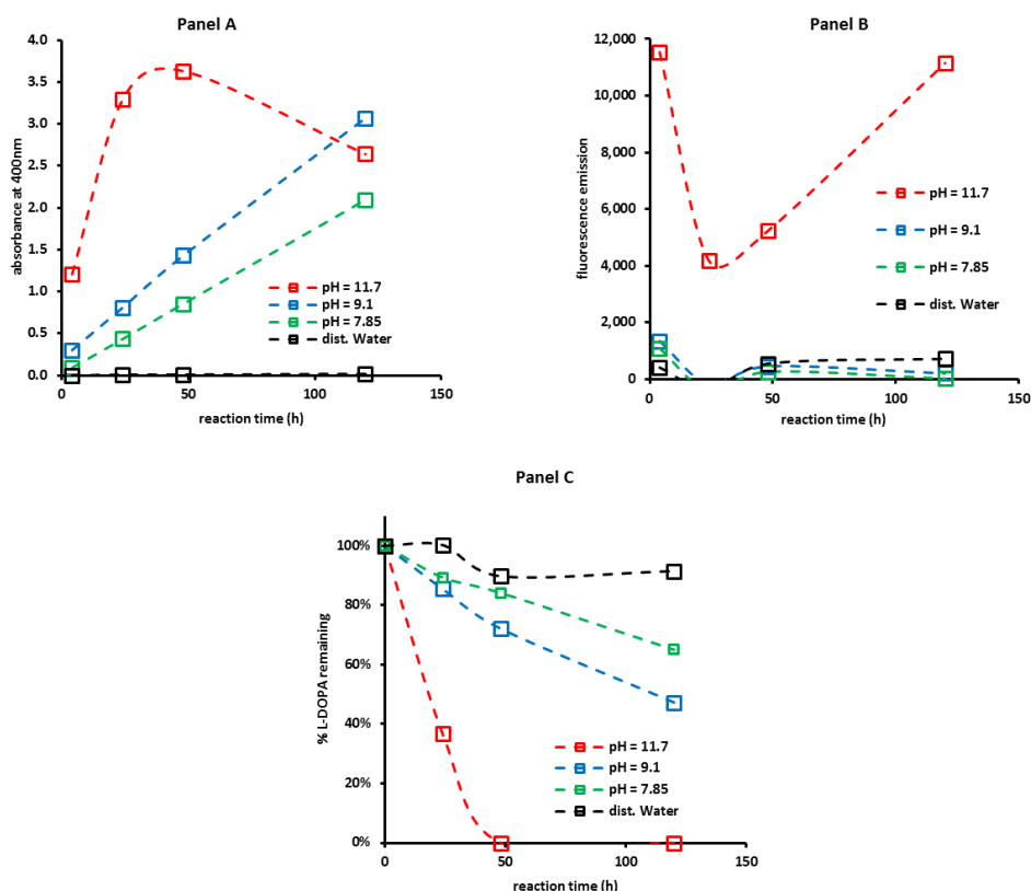
Fig.2: Kinetic profile of the changes in absorbance at 400nm (panel A), fluorescence emission (panel B) and % L-DOPA remaining (panel C) for 25mL reaction mixtures containing 25mg L-DOPA in buffers with pH values at 11.7, 9.1, 7.85 or in distilled water.
