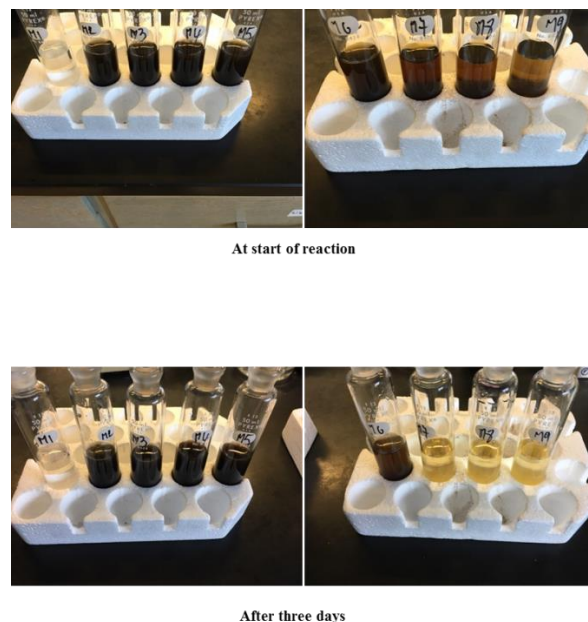
Fig. 4: Photographs of 25mL reaction mixtures containing 25mg L-DOPA, 0.3mM \text{Fe}^{2+} and, from left to right, 0, 0.01, 0.03, 0.06, 0.12, 0.24, 0.48, 0.72, 1.0% v/v \text{H}_2\text{O}_2 at the start of the experiment and after three days of reaction at RT.
