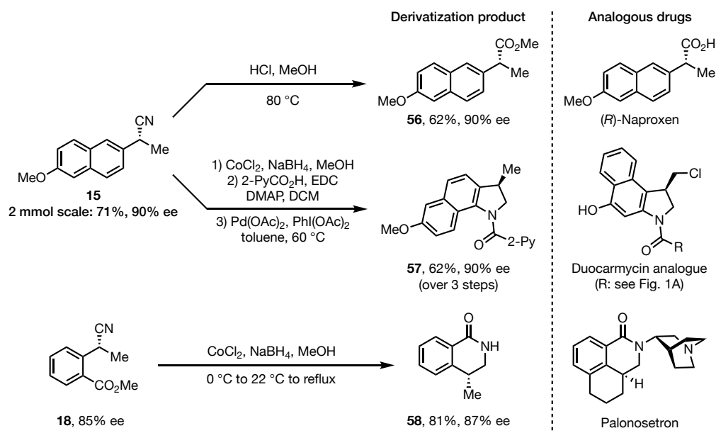
Figure 4. Product derivatization.
