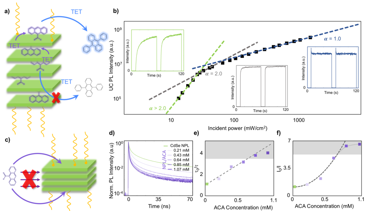
Figure 5: a) Schematic showing triplet energy transfer (TET) with stacked NPLs that have already undergone ligand exchange. While TET can occur to the ACA transmitter ligand, steric hindrance from the stacked NPLs disallows TET from buried ACA ligands to DPA. b) Plot of the UC PL intensity at different laser fluences of a sample with a high NPL concentration. There are three slope regions: a slope greater than 2 (green), where a high degree of photobrightening over time occurs (green inset), a slope of 2, (gray) where a lesser degree of photobrightening occurs (gray inset), and a slope of 1 (blue), where no photobrightening over time occurs (blue inset). c) Schematic detailing ligand exchange in prestacked NPLs. When NPLs stack, they disallow ligand exchange to occur at sites buried in the NPL stacks. d) Time-resolved PL decay in pre-stacked NPLs. e) Stern-Volmer plot utilizing the ratio of NPL lifetimes against the ACA concentration f) Stern-Volmer plot examining the ratio of steady-state intensities of the NPL emission at different ACA concentrations. A quadratic fit is shown for the first four points (dashed gray). The dotted gray line highlights the plateauing of the intensity quenching. The gray shaded region highlights the region in which the Stern-Volmer plots deviate from the expected.
