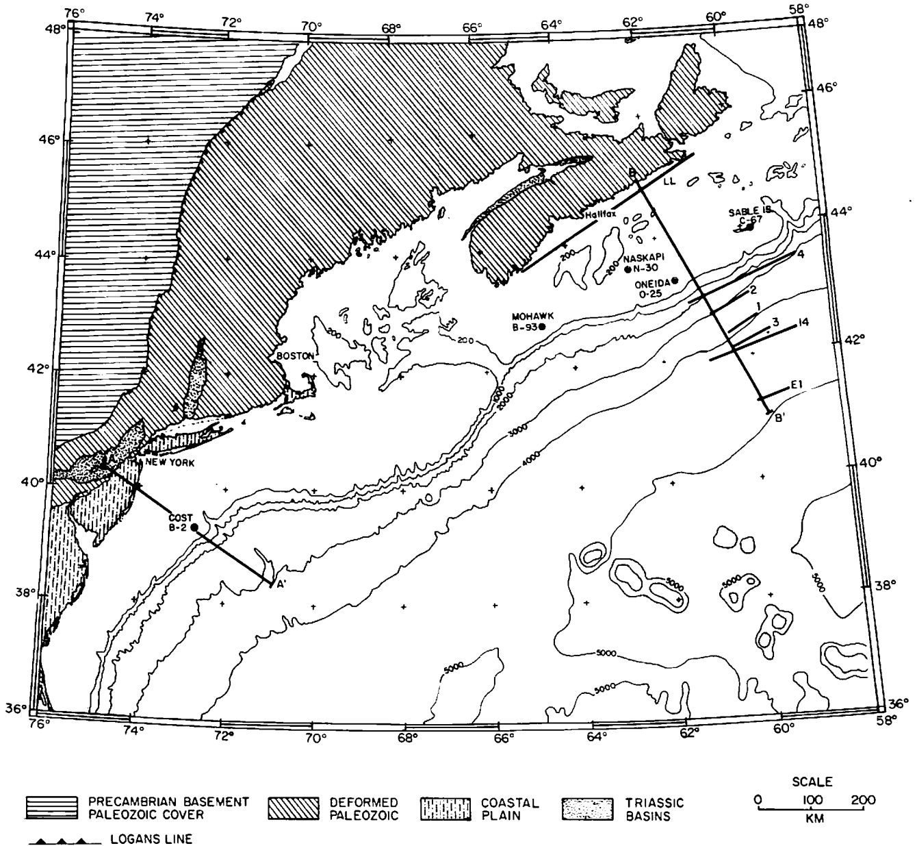
Figure 1. Location map of the COST B-2 well (Scholle, 1977) and the wells offshore Nova Scotia used in this study (Williams, 1975; Jansa and Wade, 1975; A. W. Bally, personal communication). The summary geology and generalized bathymetry are based on the tectonic map of North America (King, 1969). The heavy lines with bars indicate the location of the schematic geological structure sections of the margin shown in Figure 2 and the heavy lines without bars indicate the location of seismic refraction stations 1, 2, 3, 4 of Keen et al. (1975), E1 of Ewing and Ewing (1959), 14 of Keen and Loncarevic (1976) and LL of Barrett et al. (1964).
