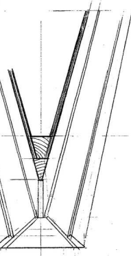
PLAN LOOKING UP OF STERN (1:5)
