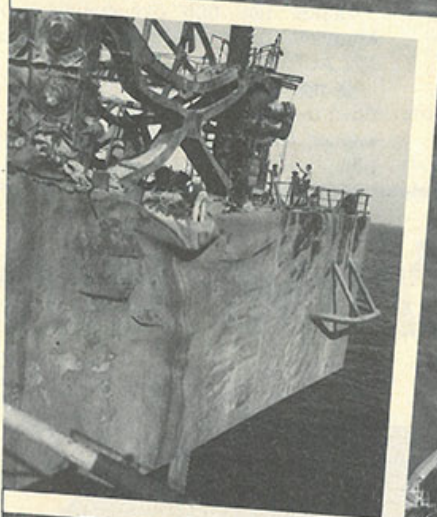
Salvage of jack-up rig "Sagar Vikas" off shore Bombay.
