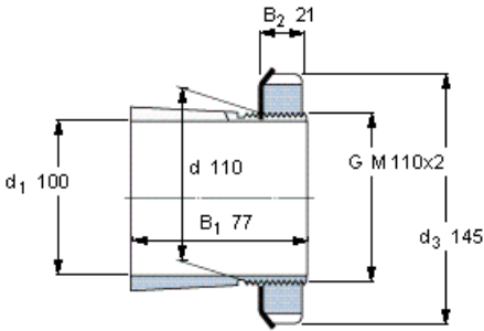
External taper of 1:12
