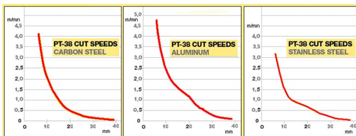
PT 38 performance with PowerCut 1600
