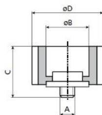
VD III for fuse base E 33
