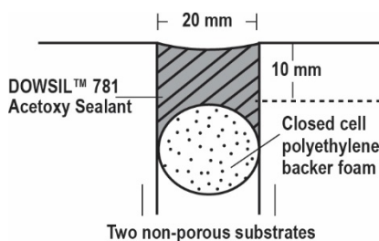
Figure 1: Deep joint
