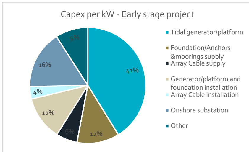
Figure 2: Capex breakdown (£/kW) for an early stage project
