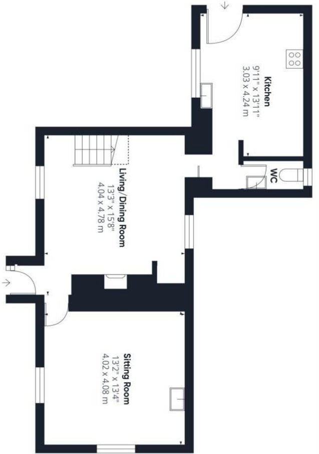
Floor 0 Building 1
