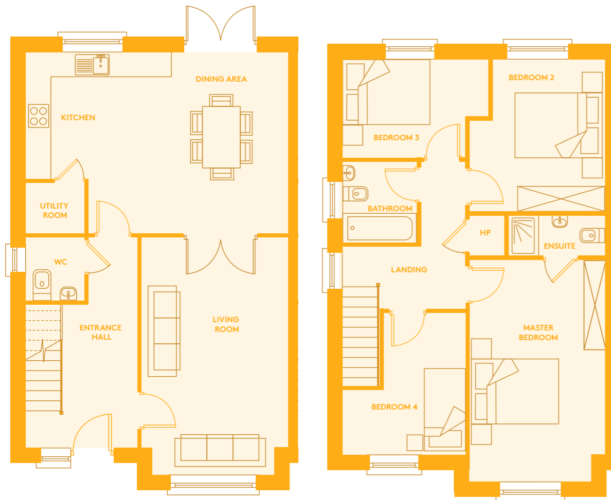
GROUND FLOOR
