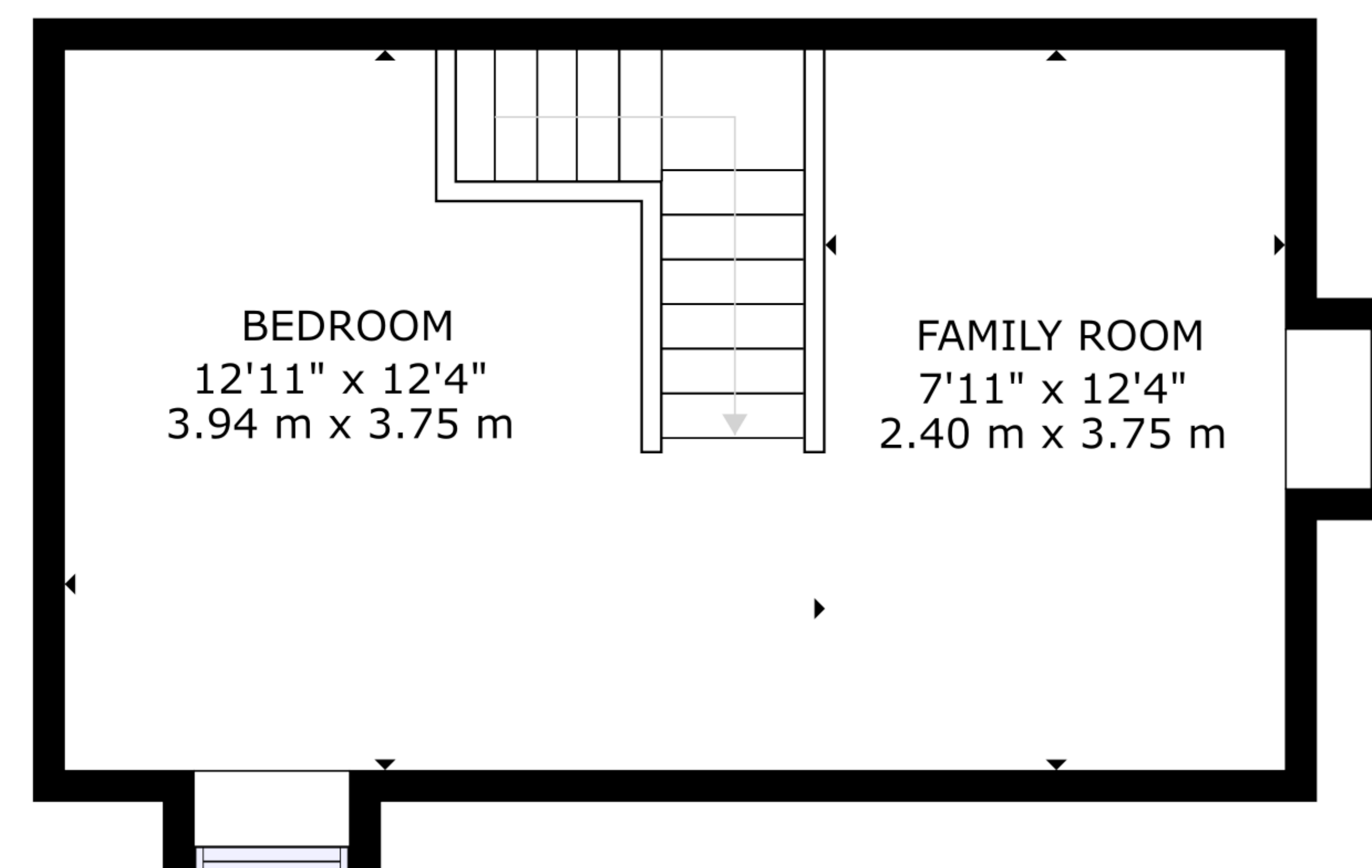
FLOOR 2
