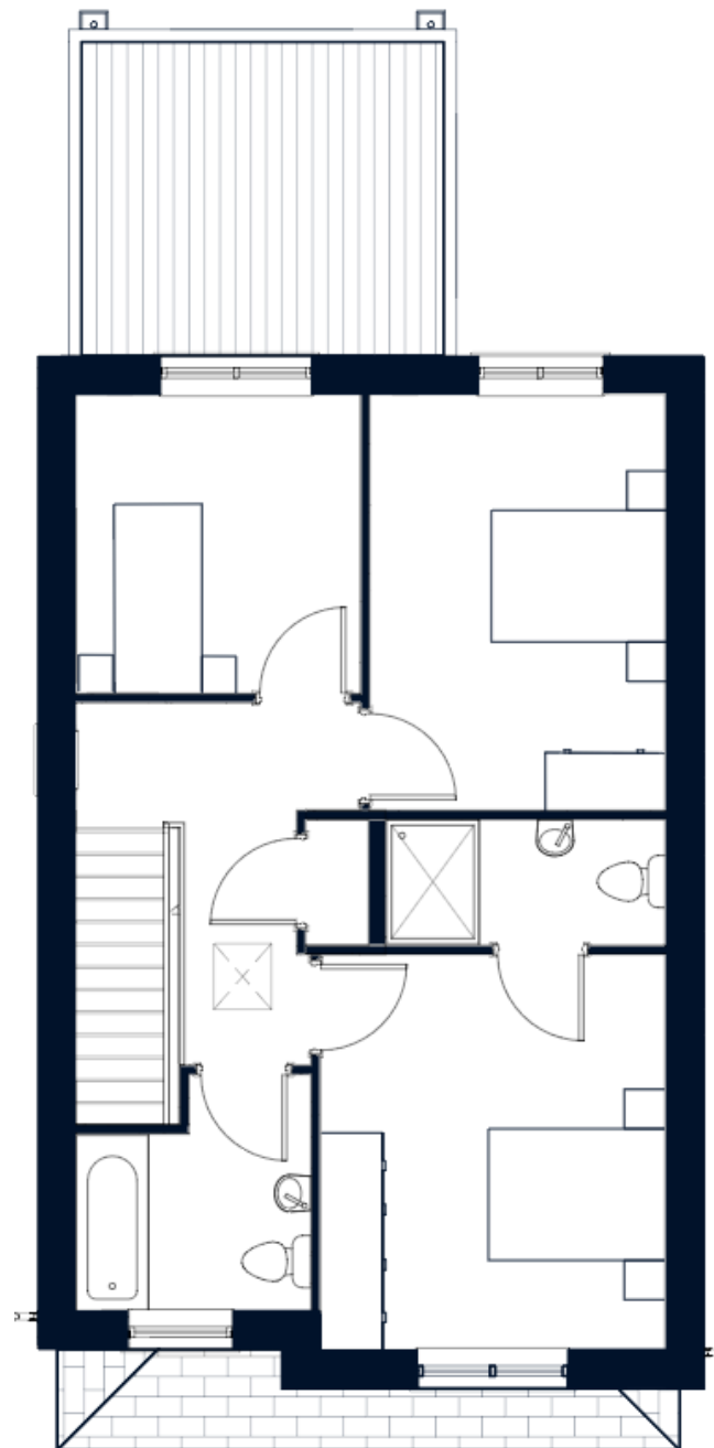
FIRST FLOOR
