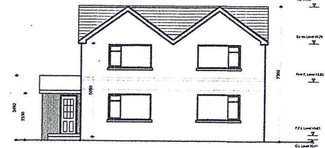
EXISTING SOUTH ELEVATION SCALE 1:200 A3
