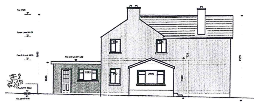
EXISTING WEST ELEVATION SCALE 1:200 A3
