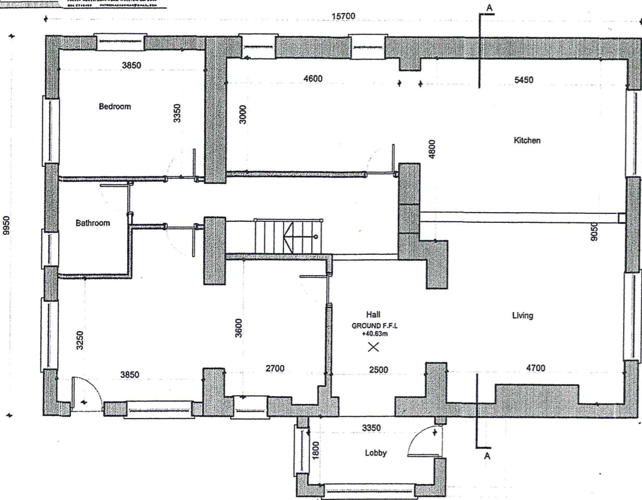
EXISTING GROUND FLOOR PLAN SCALE 1:100/1:50 A3
