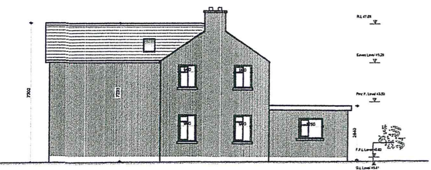
EXISTING EAST ELEVATION SCALE 1:200 A3
