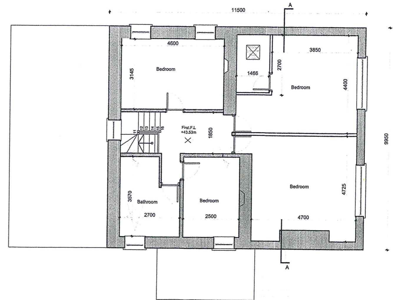
EXISTING FIRST FLOOR PLAN SCALE 1:100/1:50 A3
