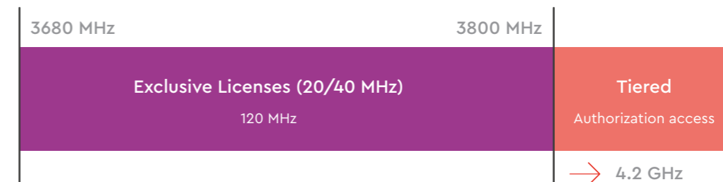
Figure 7: Status Quo
