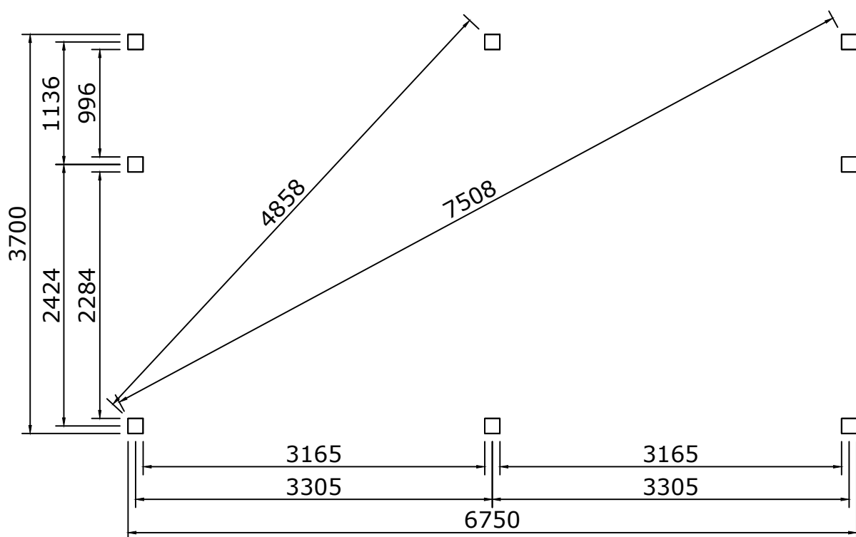
Palenplan - Floorplan - Lageplan
